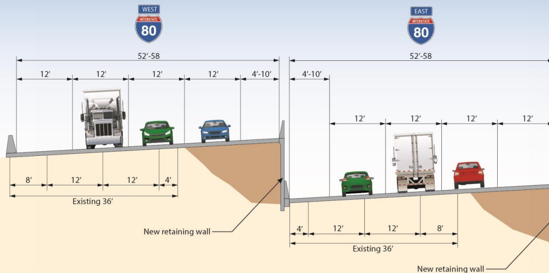
Example - Widened Roadway Cross-Section
