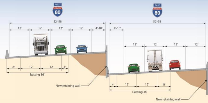
Example - Widened Roadway Cross-Section
