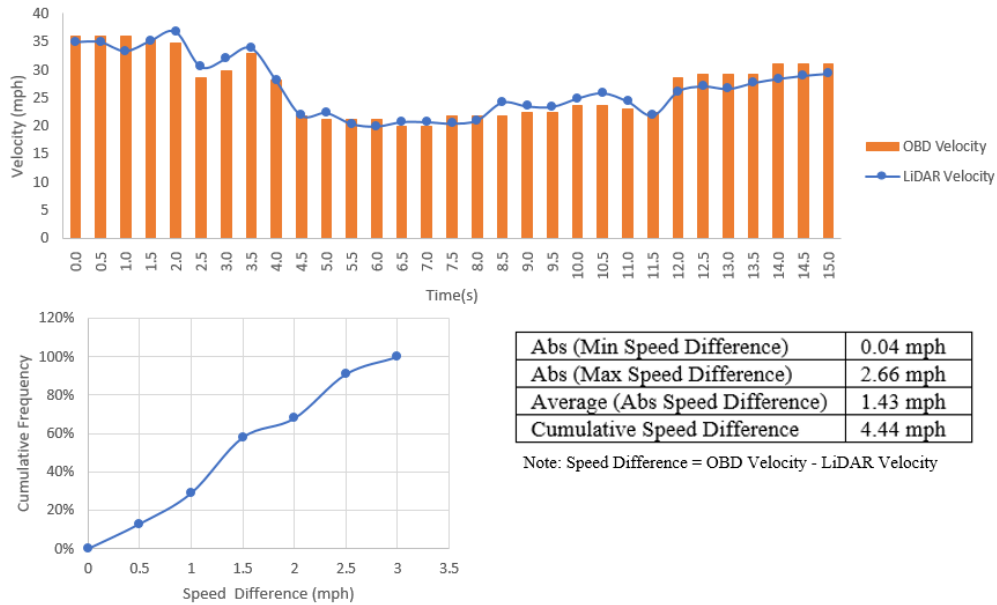
Figure 3-14 Validation of speed information extracted from roadside LiDAR
