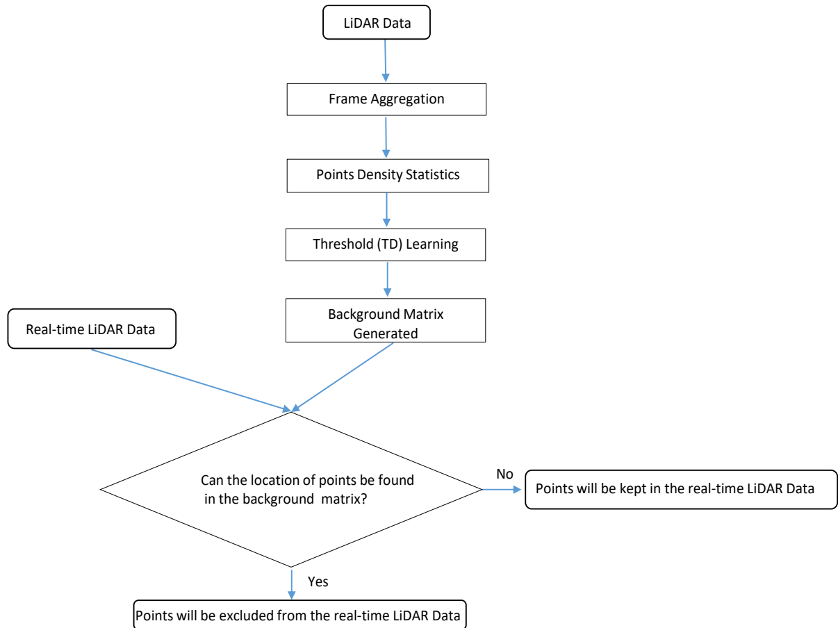
Figure 3-1 Flow chart of the developed 3D-DSF algorithm
