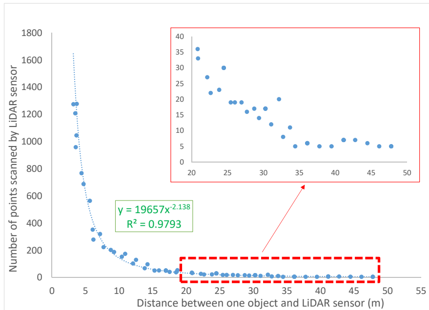
Figure 3-3-2 Distribution of vehicle points in LiDAR data
