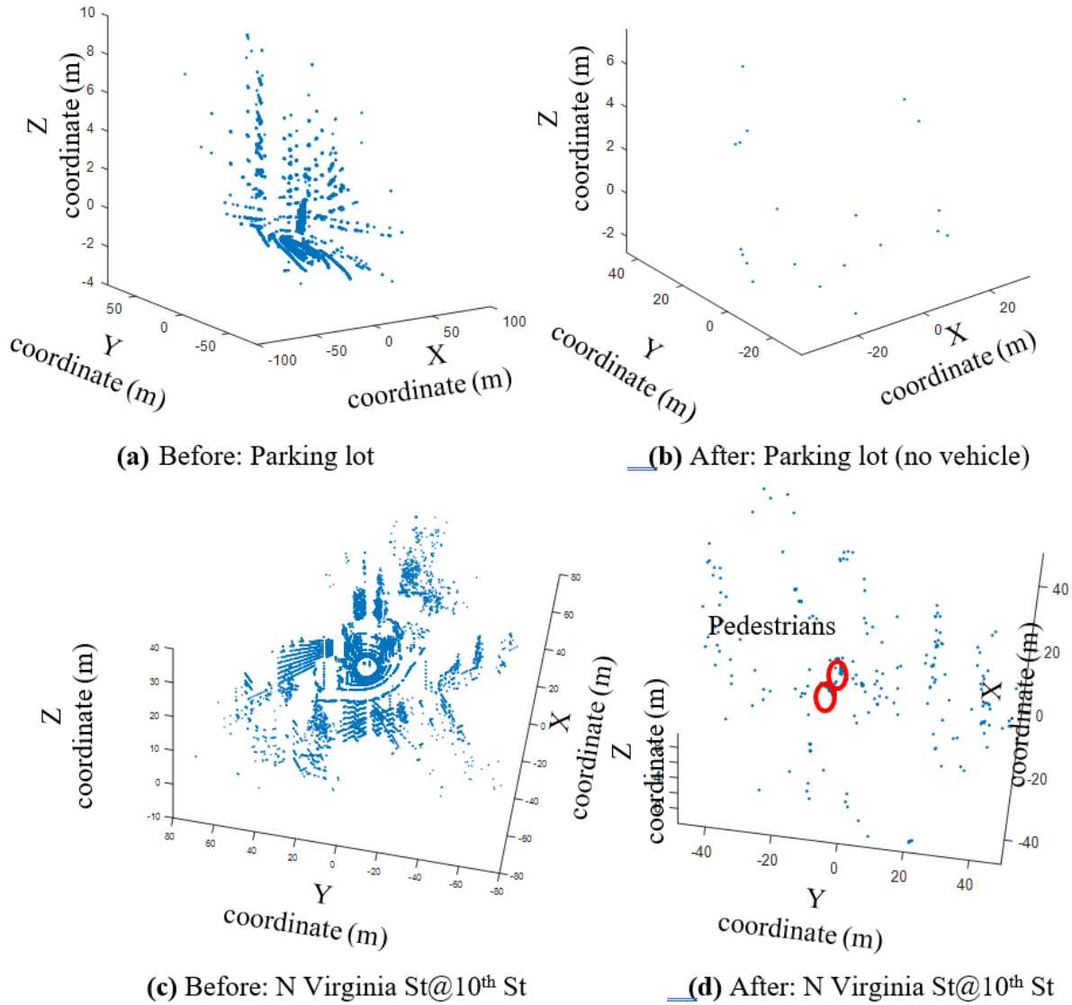
Figure 3-4 Examples of before and after background-filtering
