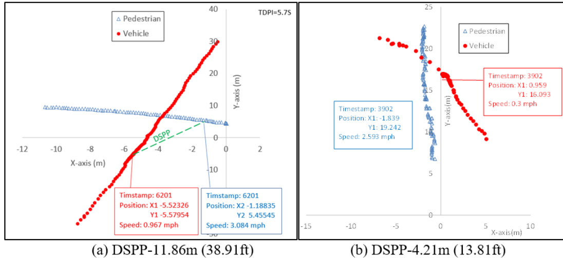
Figure 4-10 Two Different DSPP with Similar TDPI
