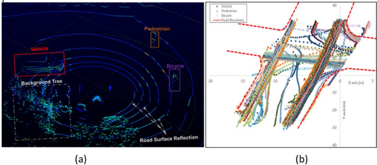
Figure 0-2 (a) Unprocessed LiDAR frame from a roadside Velodyne VLP-16 sensor, showing how resulting point-cloud data fix and can track objects precisely in three dimensions; (b) high-accuracy, multimodal traffic trajectories obtained using sequences of point cloud data from a roadside LiDAR sensor by the project team
