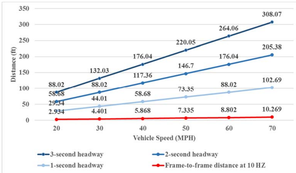
Figure 3-10 Comparison of frame-to-frame travel distance and distances between adjacent vehicles in the same lane.
