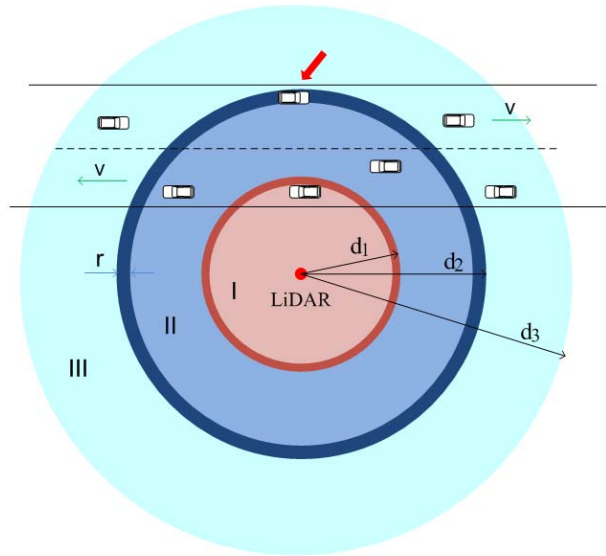
Figure 3-6 Clustering area division for using different parameters
