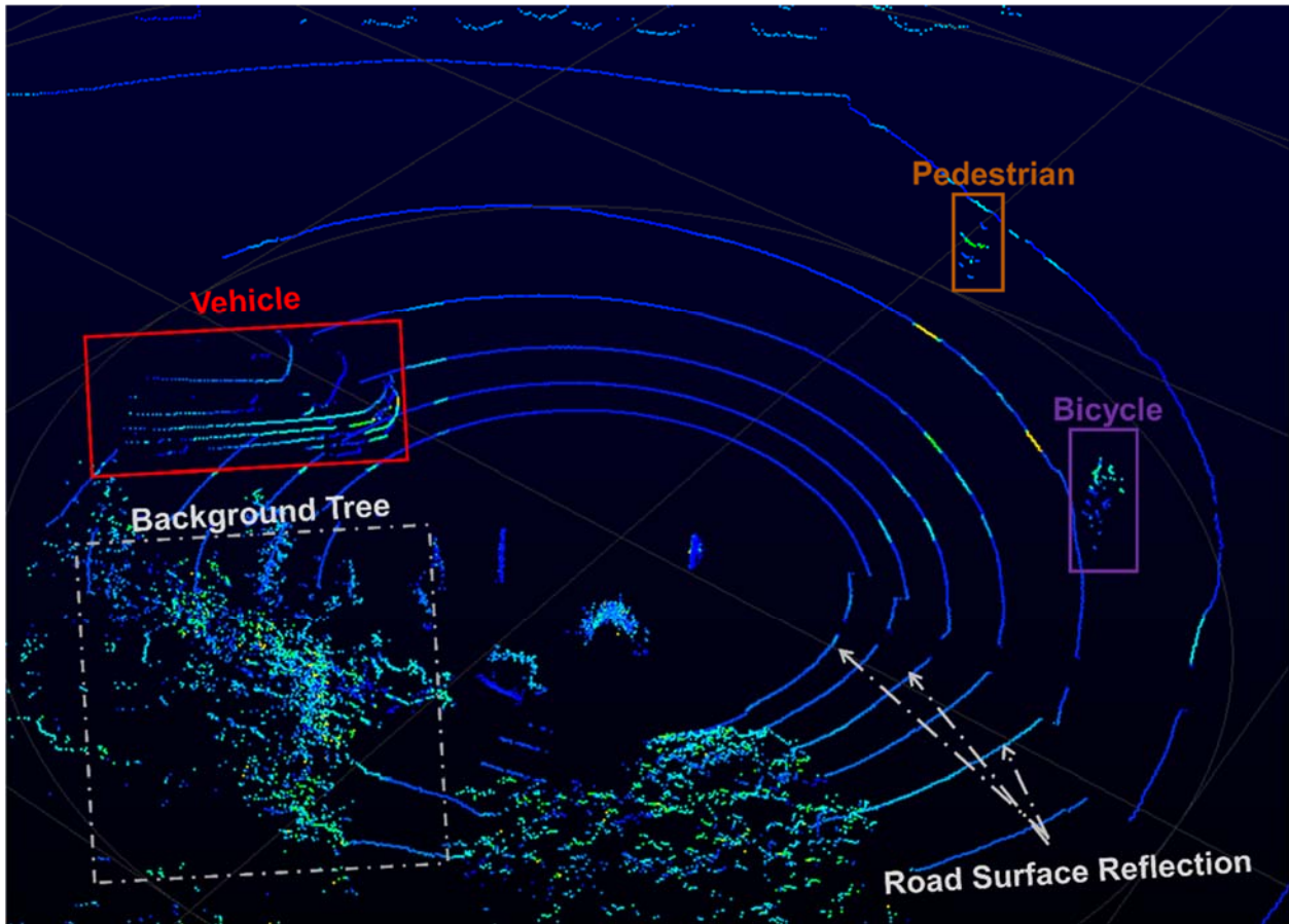
Figure 1-1 Demonstration of a 360-degree LiDAR data frame
