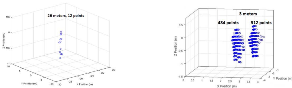
(a) Pedestrian data points at 26 meters from LiDAR. (b) Pedestrian data points at 3 meters from LiDAR. Figure 3-5 Comparison of obtained points from pedestrians at different distances from a VLP-16 sensor
