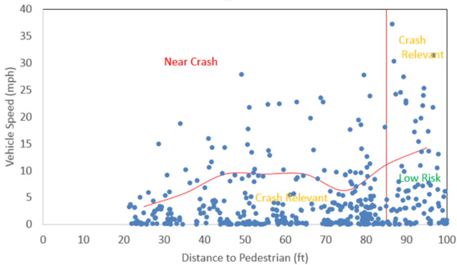
(c) Speed-Distance Profile
