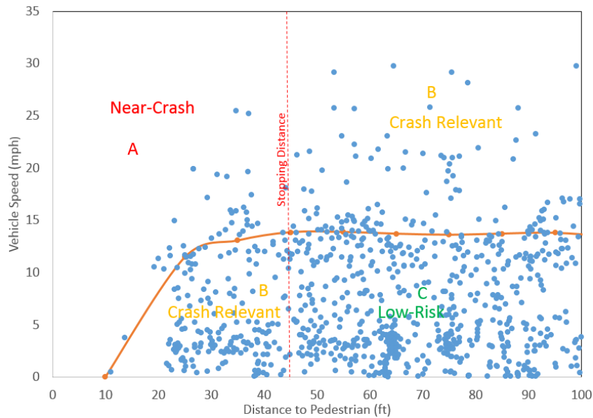
Figure 4-12 An Example of Near-Crash Identification with Speed-Distance Profile
