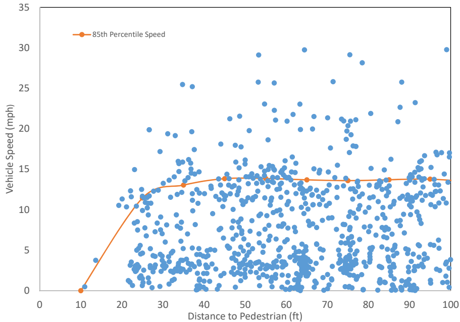
Figure 4-11 Speed-Distance Profile of Vehicles
