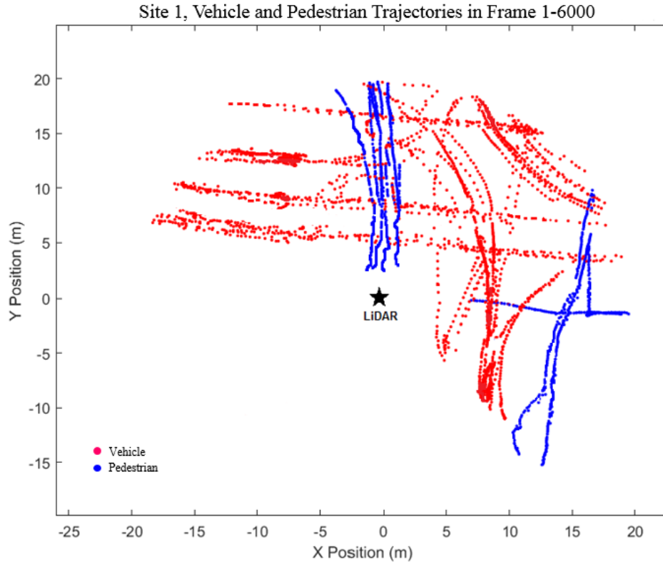
Figure 3-13 Example of extracted vehicle and pedestrian trajectories
