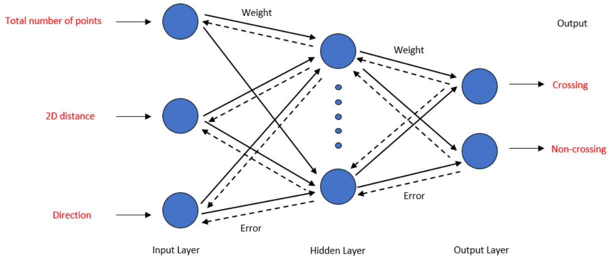
Figure 3-8 Structure of BP-ANN model
