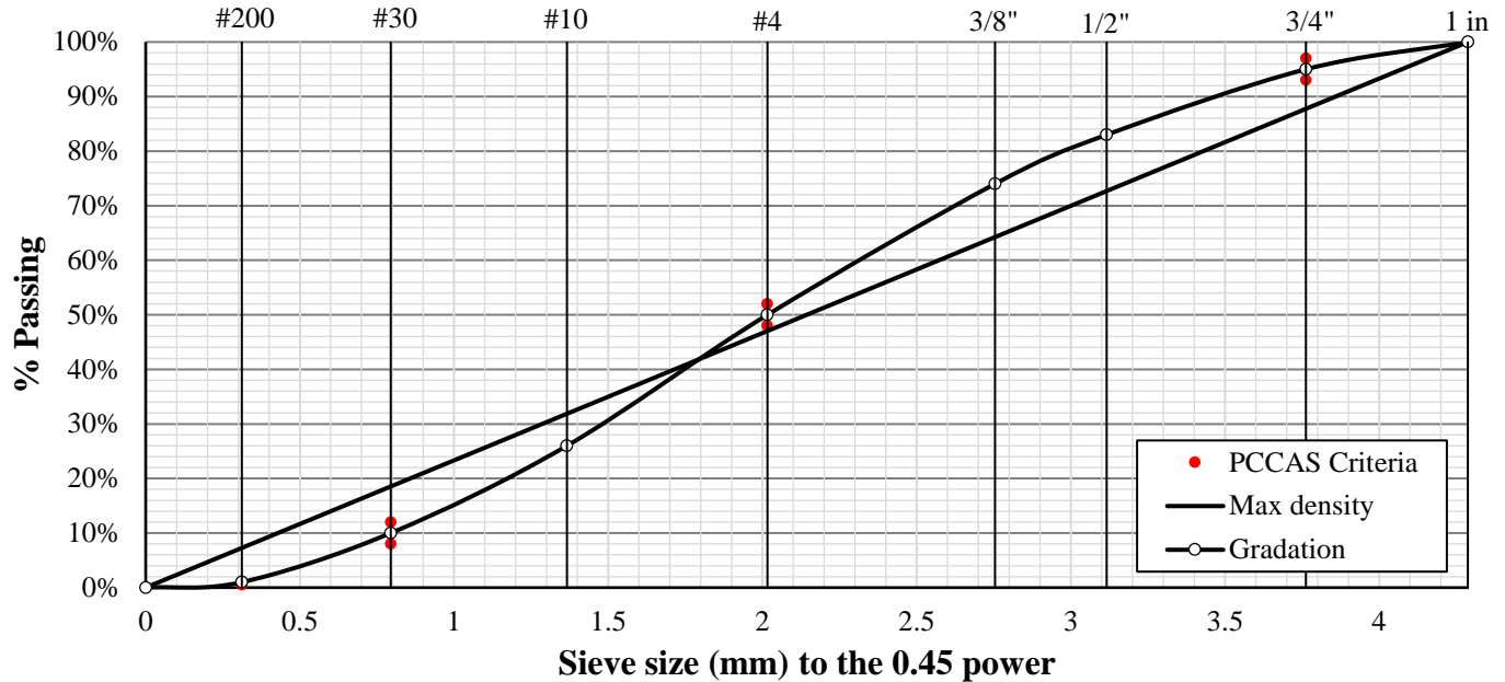
Figure 3.1. Gradations of the graded RAP materials.
