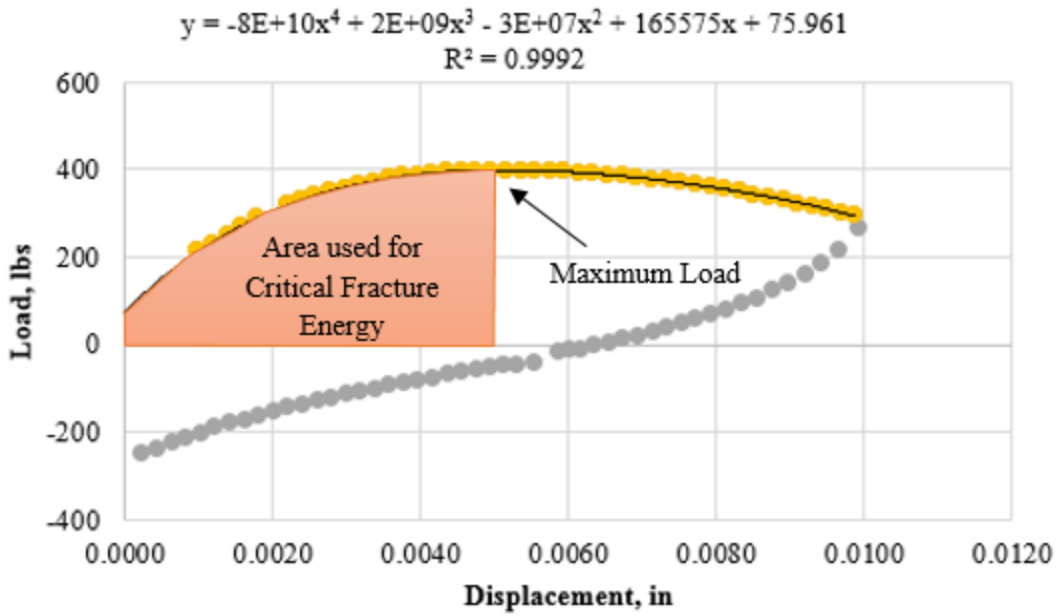
Figure 4.15. Hysteresis loop for CIR mixture under the first OT cycle.
