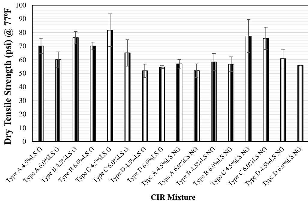
Figure 3.11. Dry TS properties of CIR mixtures designed with the Superpave method.
