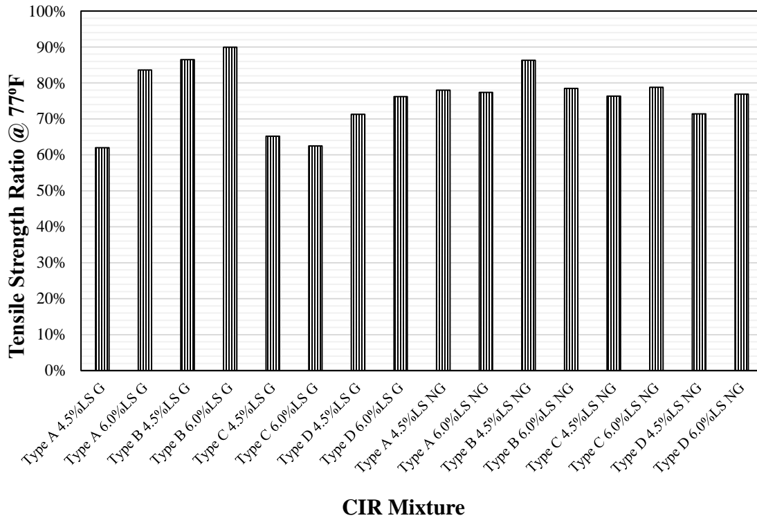
Figure 3.13. Tensile strength ratios of CIR mixtures designed with the Superpave method.
