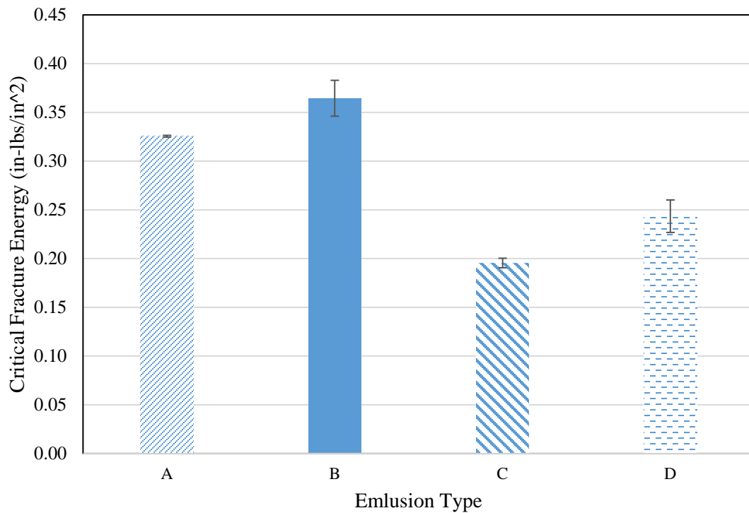
Figure 4.18. Crack initiation of CIR mixtures; non-graded RAP and 6.0% lime slurry.
