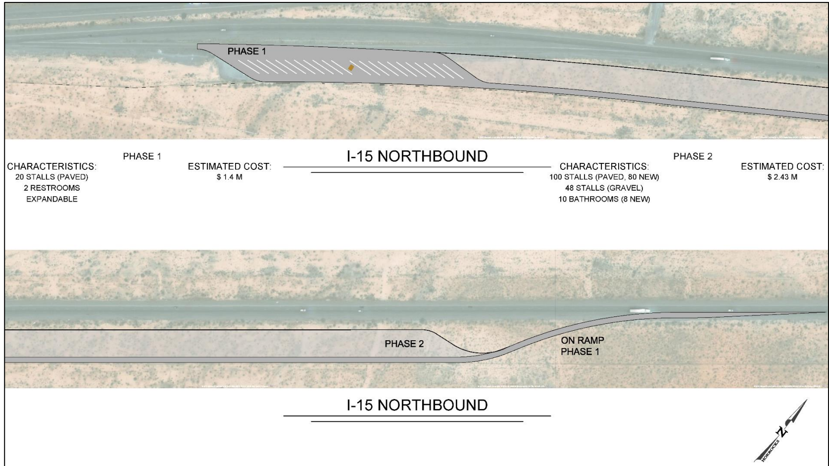
Figure 4.9 MP 96 Truck Turnout Expansion, I-15 Northbound
