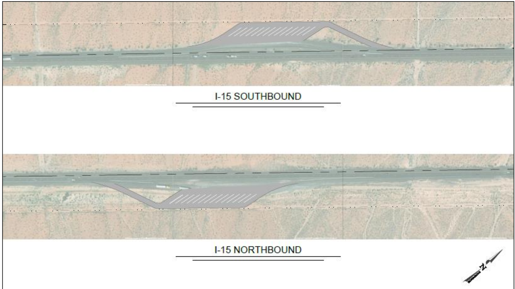
Figure 4.10 MP 88 Truck Turnout Expansion, I-15 $1,150,000 for an additional 26 regular spaces
