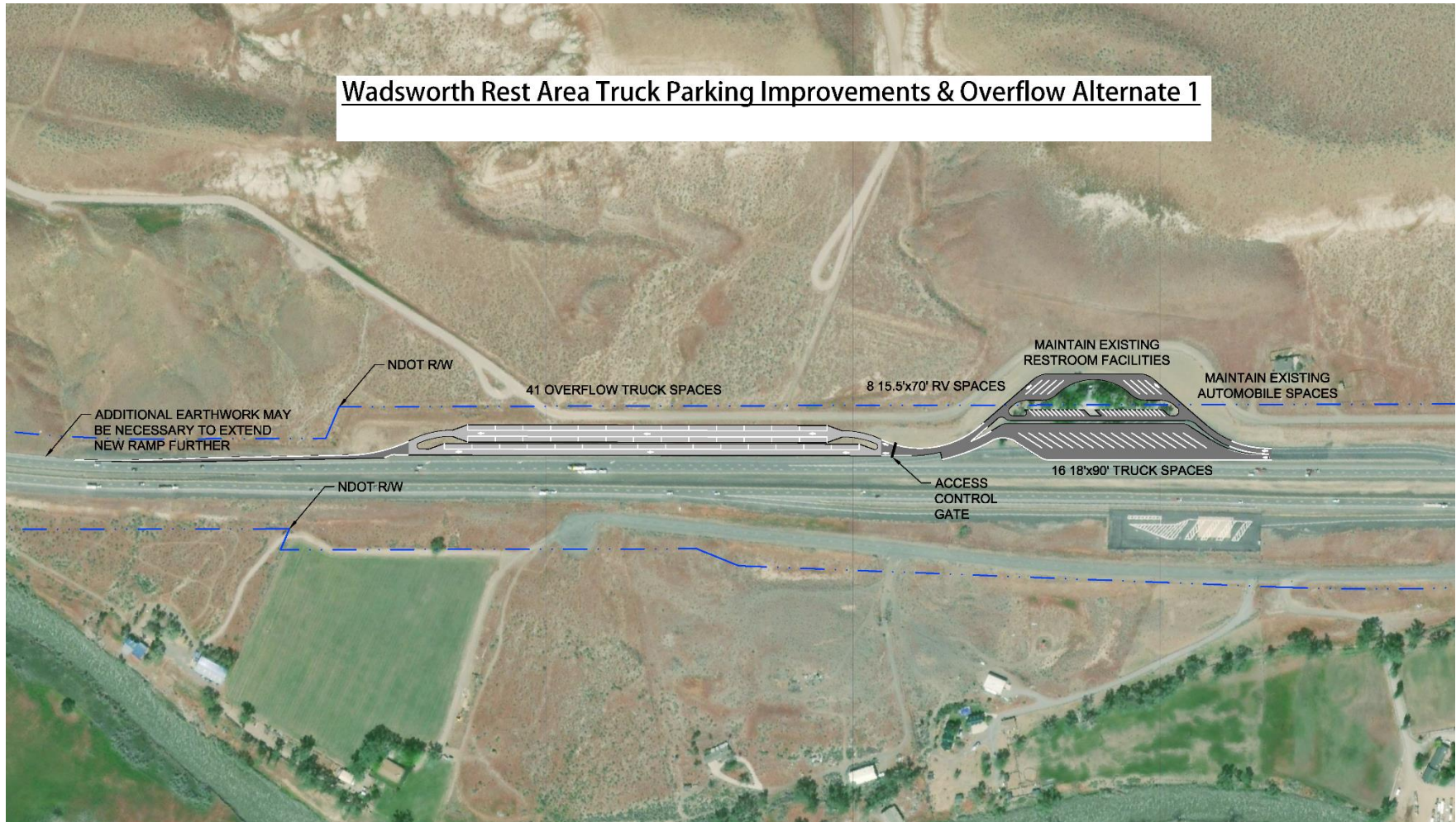
Figure 4.2 Wadsworth Rest Area Expansion, I-80 $1,227,000 for an additional 10 regular and 41 emergency spaces
