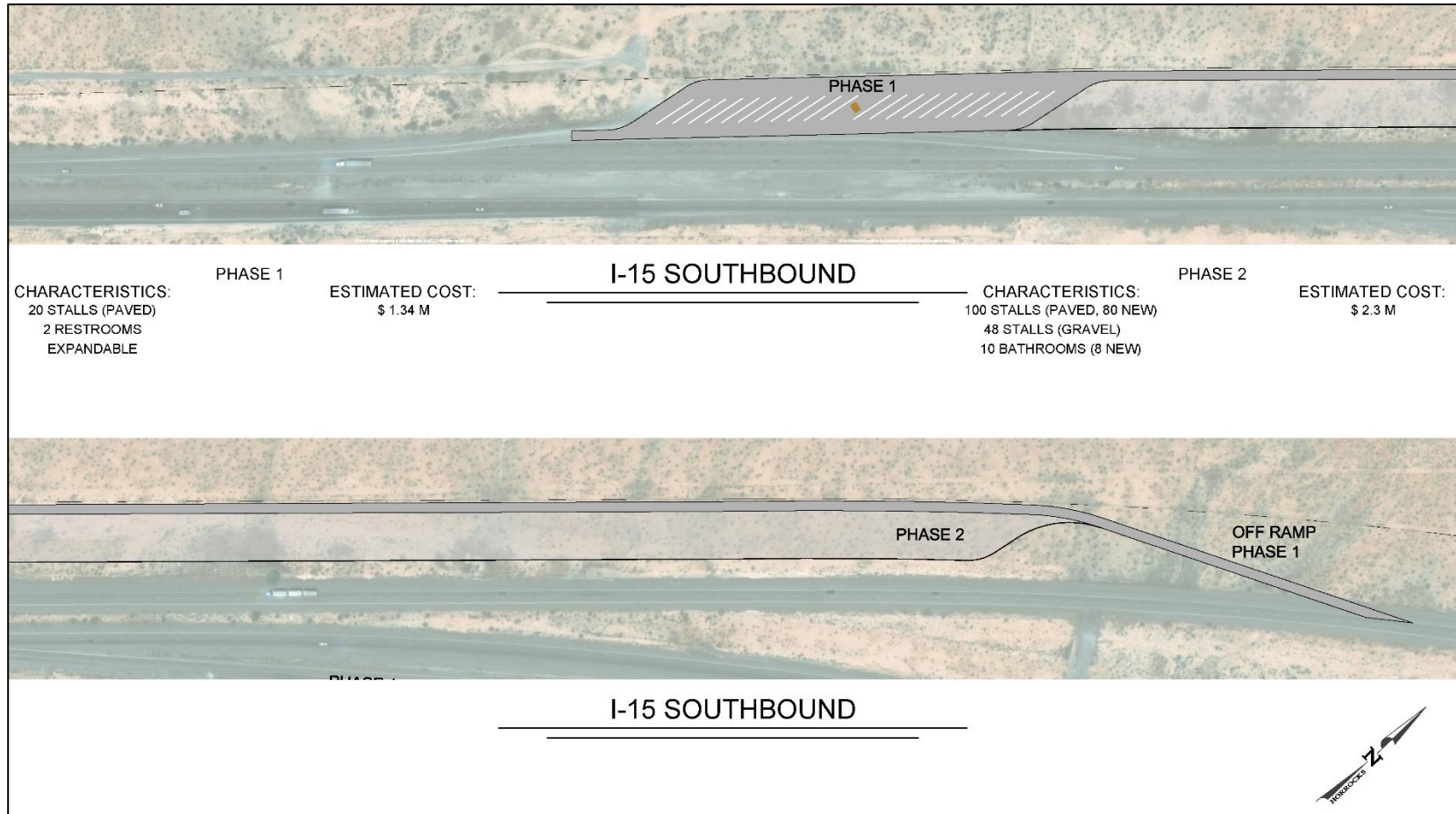
Figure 4.8 MP 96 Truck Turnout Expansion, I-15 Southbound
