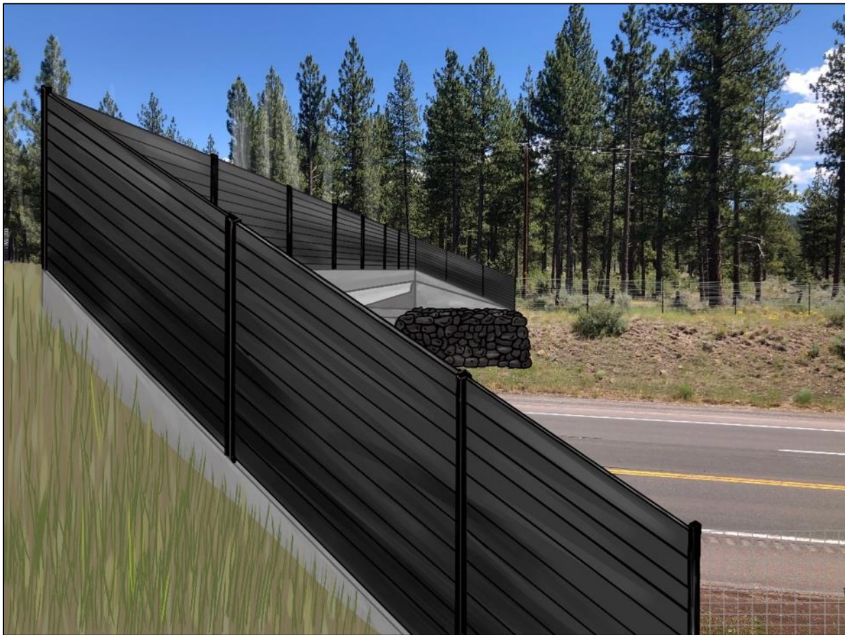
Figure 16: Recycled-plastic sound and light barrier installed on top of soil-retaining concrete curb.
