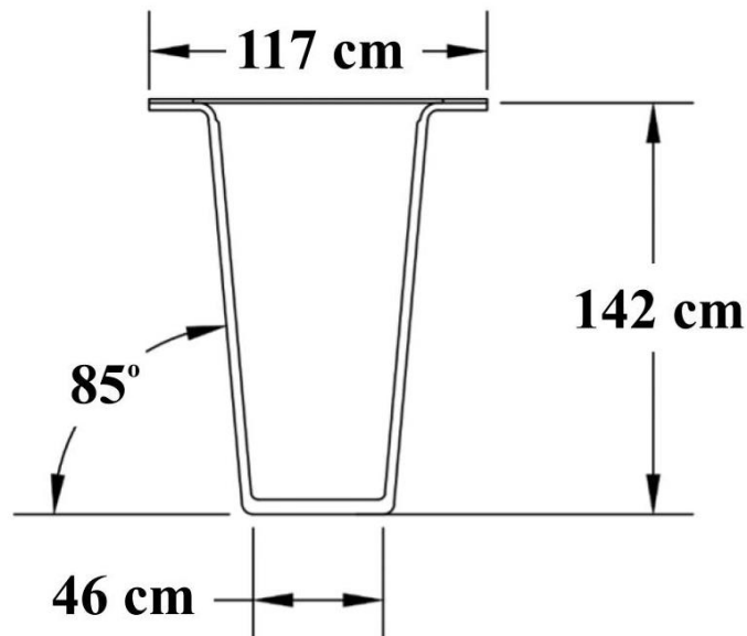
Figure 14: Cross section of the preliminary design for the CT girder from AIT Bridges.
