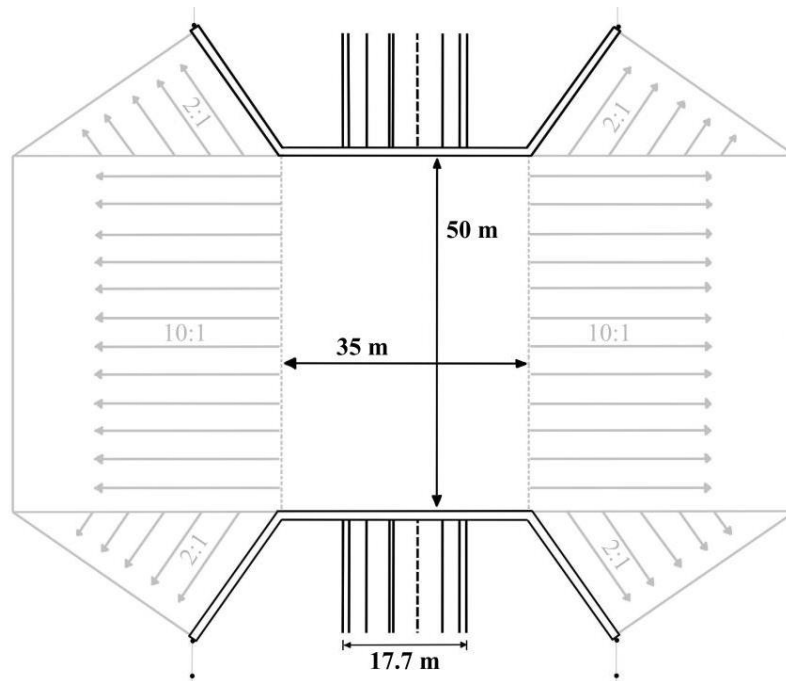
Figure 10: Plan view with dimensions of the US-97 wildlife overpass.
