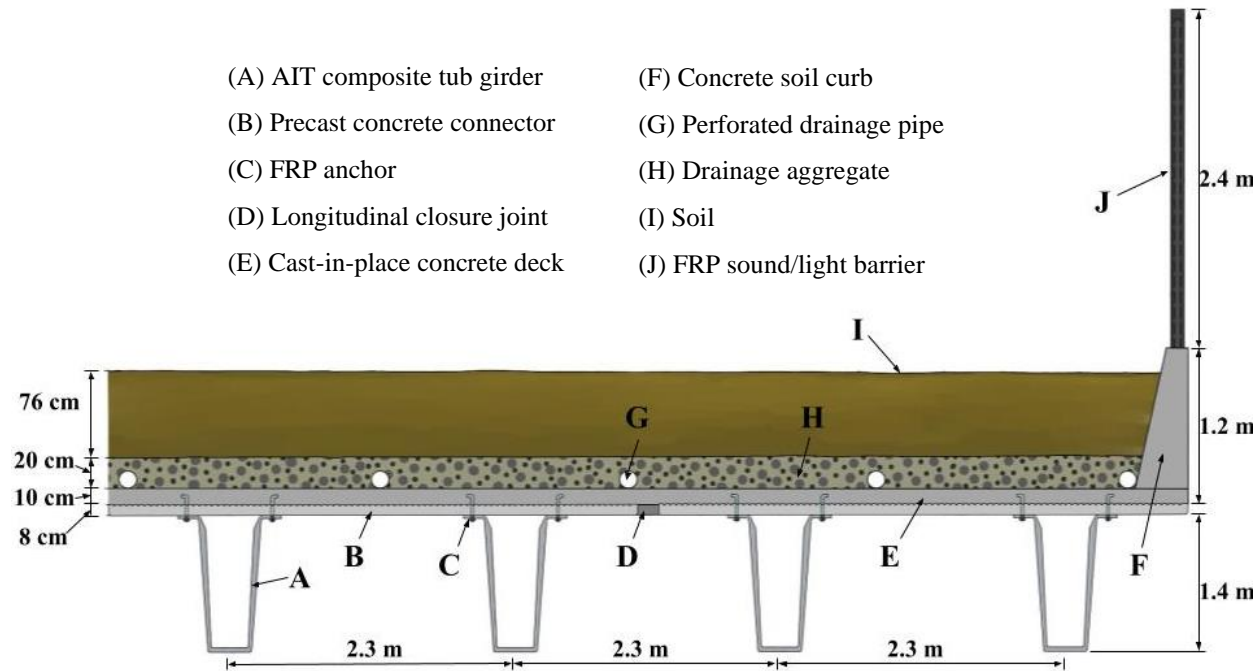
Figure 15: Cross section of the wildlife overpass showing the layout of the girders, concrete deck, soil, drainage, and barriers on the bridge span.
