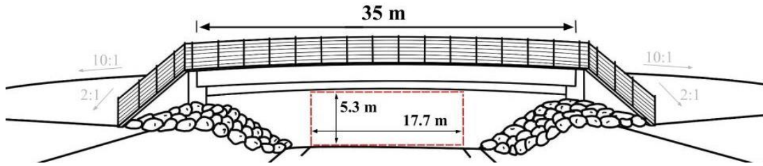
Figure 9: Elevation view of the US-97 wildlife overpass.
