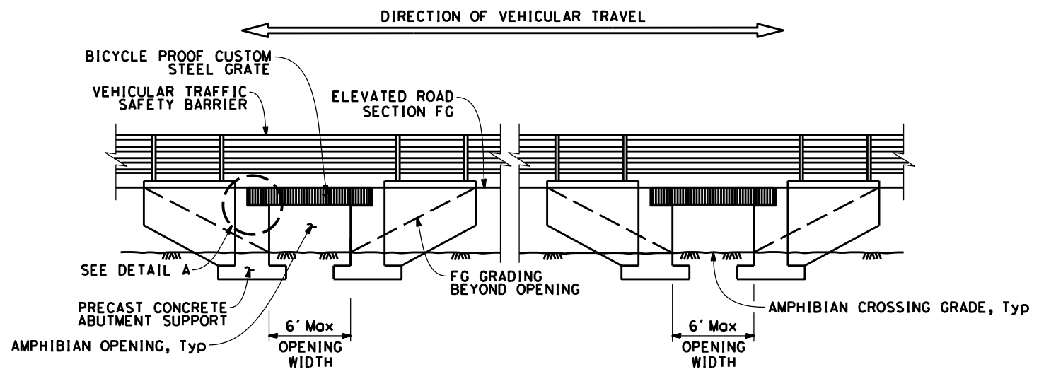
ELEVATION VIEW SCALE: 1" = 10'
