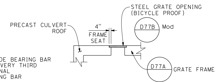
STEEL GRATE OPENING DETAIL
