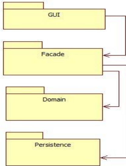
Figure 1. Class Diagram.
