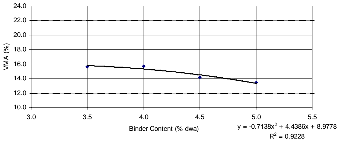
Figure 16 Percent VMA for the Lockwood Aggregate Source.
