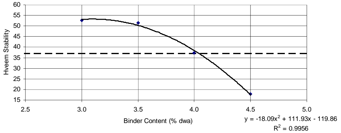
Figure 17 Hveem Stability for the Sloan Aggregate Source.
