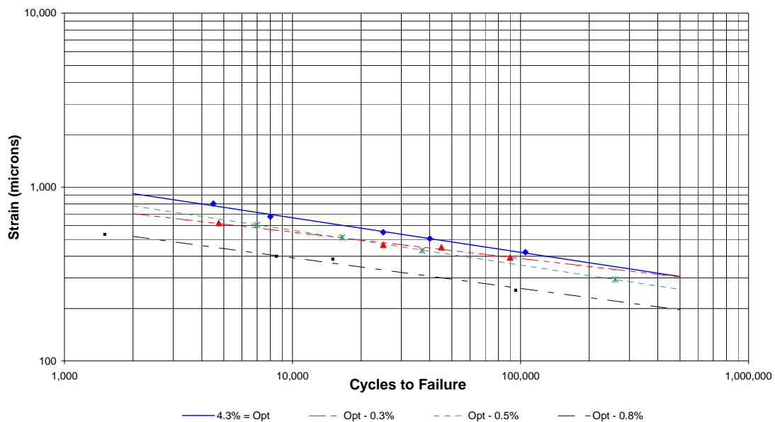
Figure 8 Comparison of Fatigue Life of the Lockwood Source at Different AC Levels.
