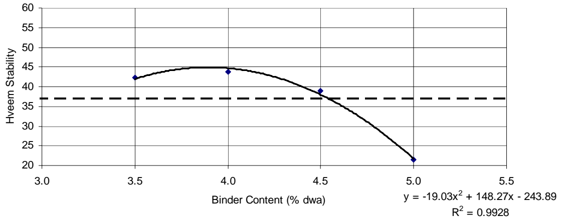
Figure 13 Hveem Stability for the Lockwood Aggregate Source.
