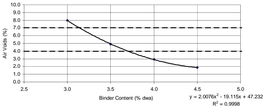
Figure 18 Percent Air-Voids for the Sloan Aggregate Source.
