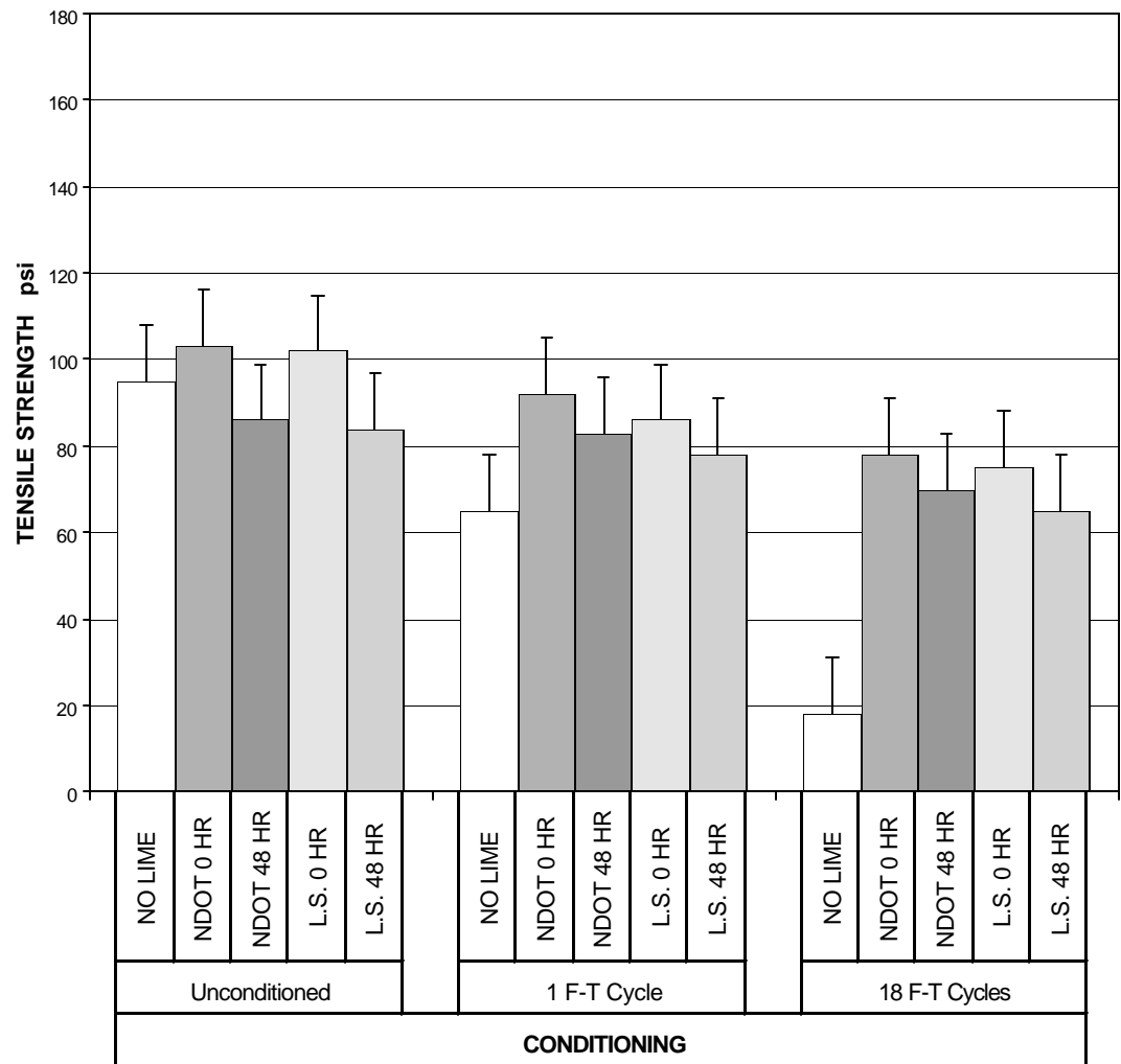
Figure 17. Average tensile strength property of the Lockwood PG 64-34 mixtures, vertical bars indicate the range of average value plus one least significant difference.
