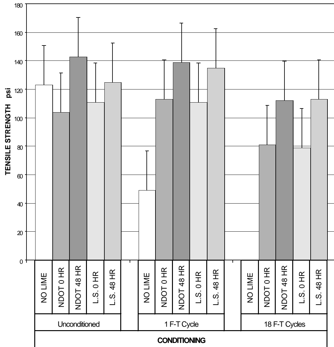
Figure 13. Average tensile strength property of the Lockwood AC-20P mixtures, vertical bars indicate the range of average value plus one least significant difference.
