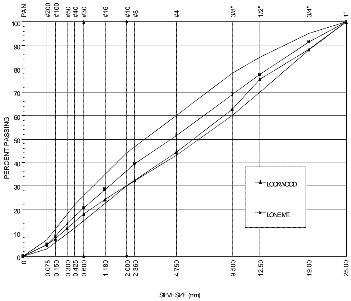
Figure 12. Gradation curves for the Lockwood and Lone Mountain aggregate sources in comparison to the NDOT Type 2C gradation specifications.
