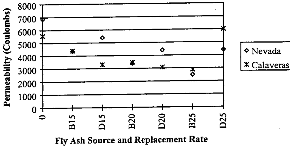
Figure 4.23 - Effect of Cement Source on 56-Day Permeability of All-Lite Aggregate Concrete
