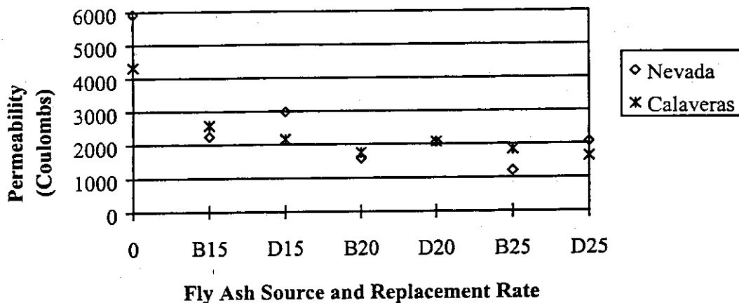
Figure 4.26 - Effect of Cement Source on 120-Day Permeability of All-Lite Aggregate Concrete
