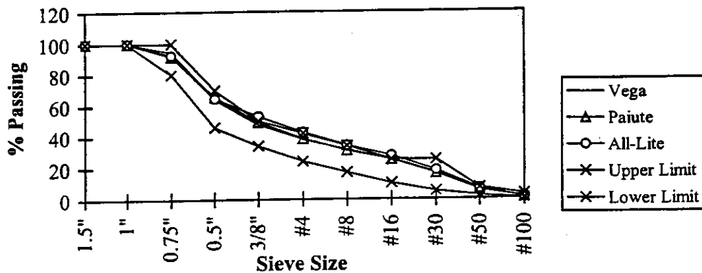
Figure 3.5 - Combined Aggregate Gradations
