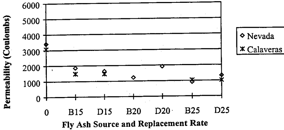
Figure 4.24 - Effect of Cement Source on 120-Day Permeability of Vega Aggregate Concrete
