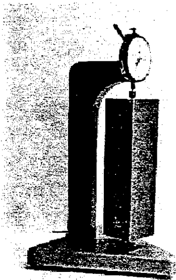
Figure 2.1 - Length Comparator with Shrinkage Specimen
