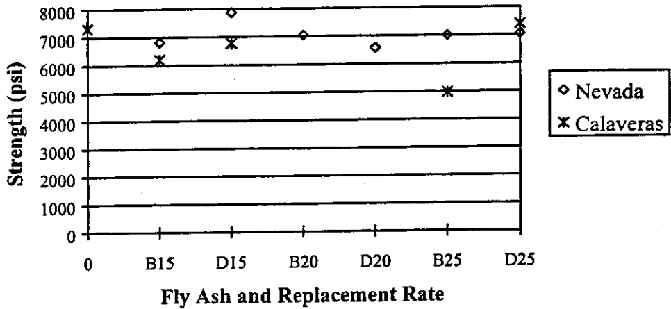
Figure 4.2 - 56-Day* Strengths for Vega Aggregate Concrete *Actual test age is greater than 56 days.
