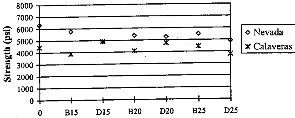
Figure 4.3 - 28-Day Strengths for All-Lite Aggregate Concrete
