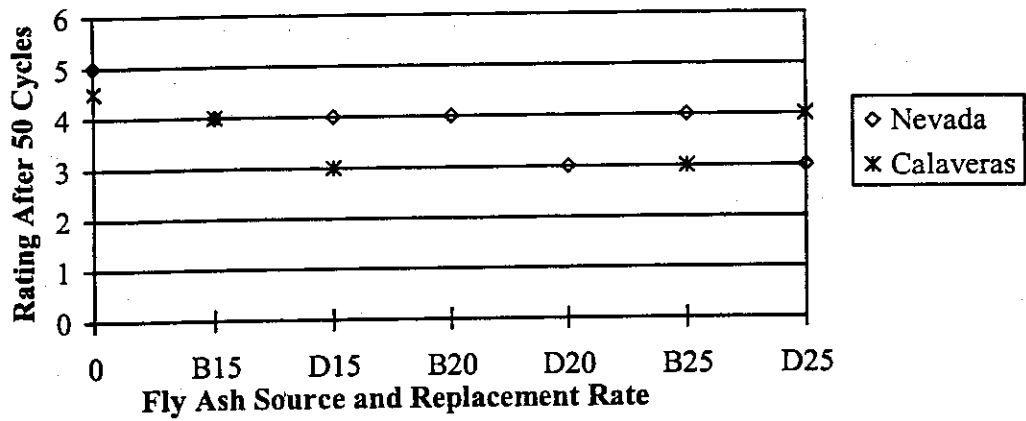
Figure 4.12 - Scaling Resistance: Effect of Cement Source with Vega Aggregate
