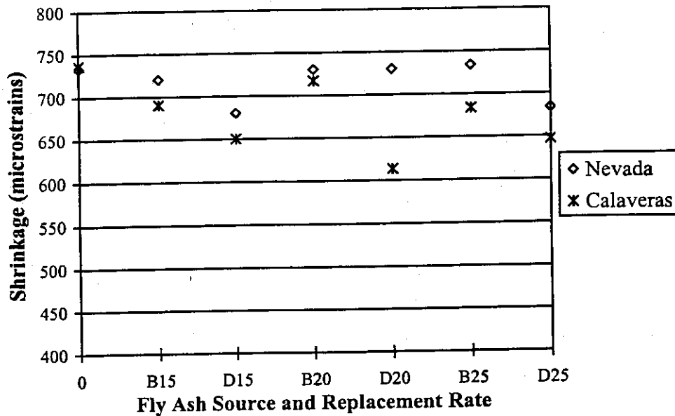
Figure 4.31 - Shrinkage of All-Lite Aggregate Concrete (16 weeks)
