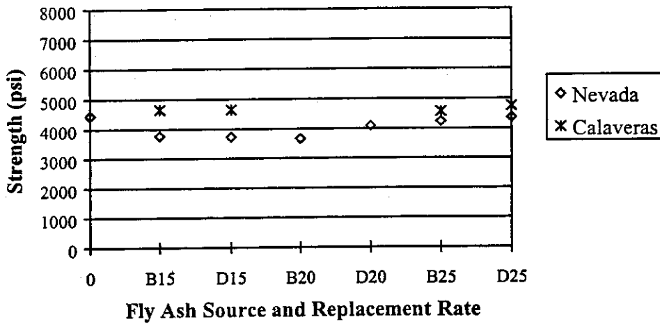
Figure 4.5 - 28-Day Strengths of Paiute Aggregate Concrete
