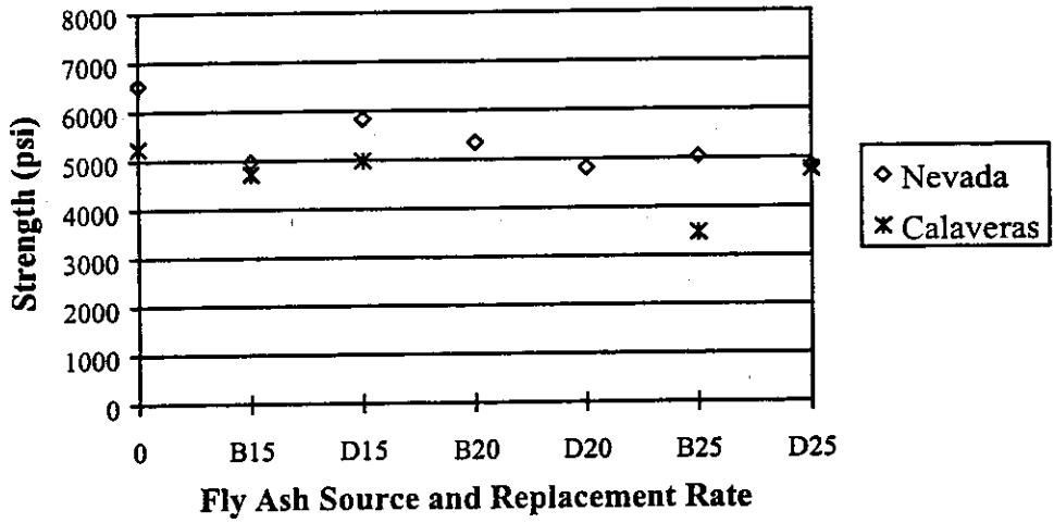
Figure 4.1 - 28-Day Strengths for Vega Aggregate Concrete
