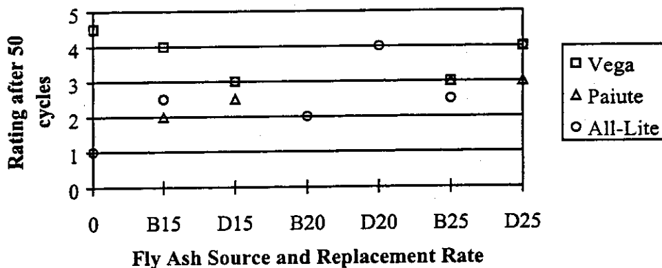
Figure 4.16 - Scaling Resistance: Effect of Aggregate Source with Calaveras Cement
