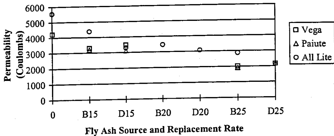
Figure 4.17 - Effect of Fly Ash on the 56-Day Permeability of Calaveras Cement Concrete
