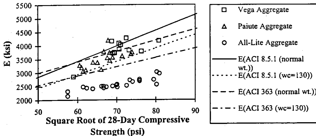
Figure 4.11 - Effect of Coarse Aggregate Source on Elastic Modulus
