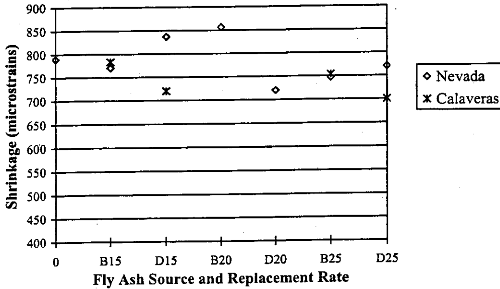
Figure 4.30 - Shrinkage of Paiute Aggregate Concrete (16 weeks)
