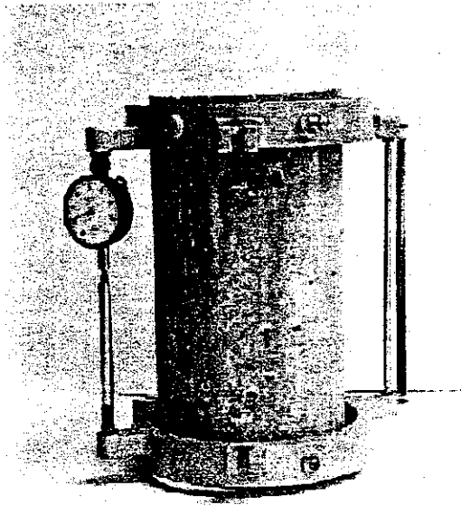
Figure 2.4 - Compressometer
