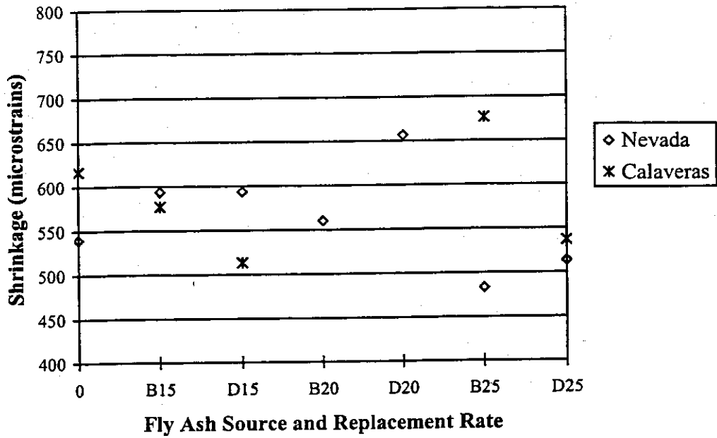
Figure 4.29 - Shrinkage of Vega Aggregate Concrete (16 weeks)
