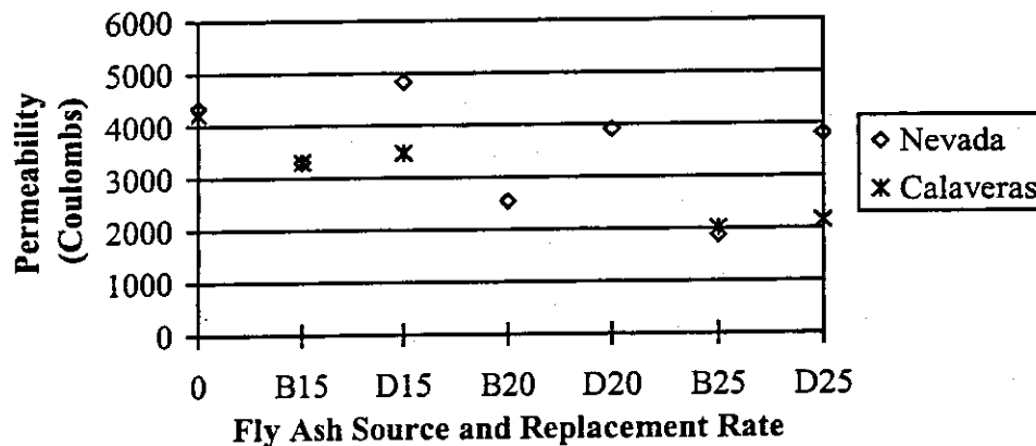
Figure 4.21 - Effect of Cement Source on 56-Day Permeability of Vega Aggregate Concrete
