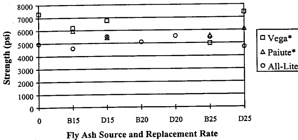
Figure 4.10 - 56-Day Strength for Calaveras Cement Concrete
