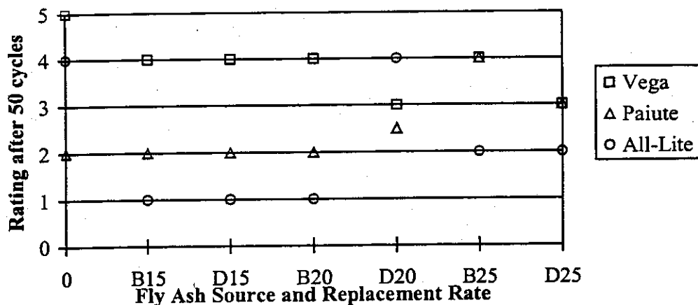
Figure 4.15 - Scaling Resistance: Effect of Aggregate Source with Nevada Cement
