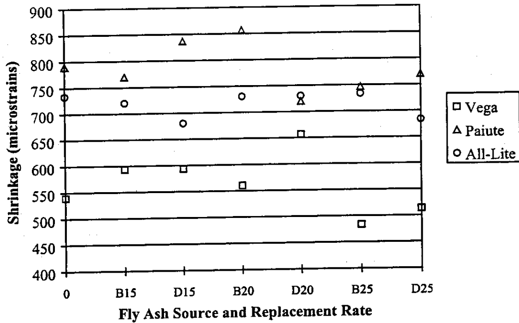
Figure 4.28 - Shrinkage of Nevada Cement Concrete (16 weeks)
