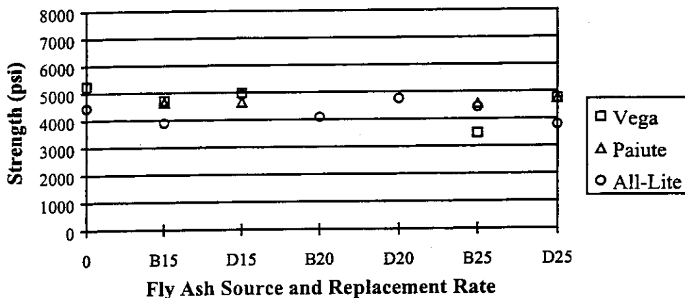
Figure 4.9 - 28-Day Strengths of Calaveras Cement Concrete
