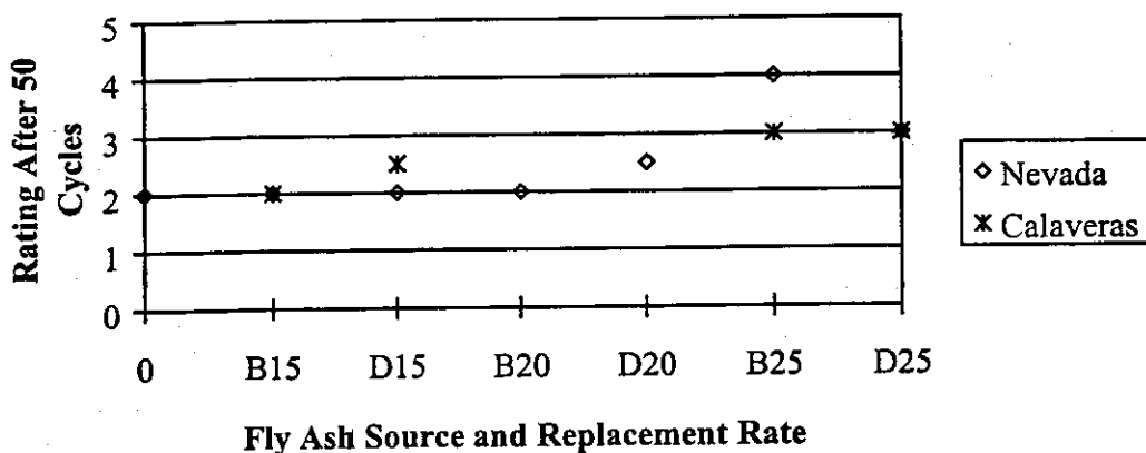
Figure 4.14 - Scaling Resistance: Effect of Cement Source with Paiute Aggregate
