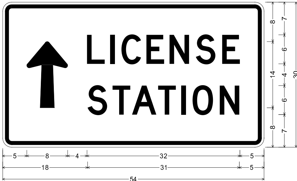
RNV9-3_54x30; 2" Radius, 1" Border, 1" Indent, Black on White; Arrow 6-2LV - 14" 90°; "LICENSE" D; "STATION" D;
