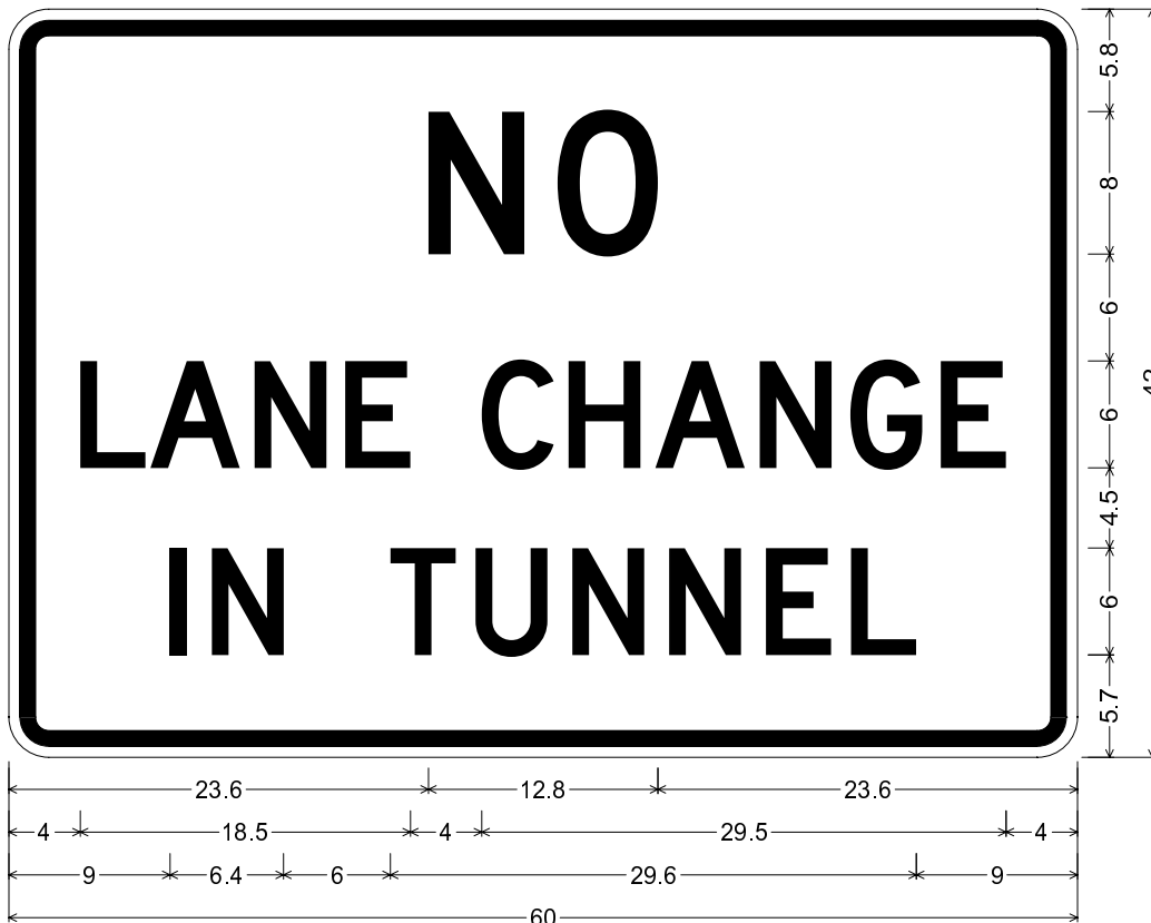
RNV5-1_60x42; 2.3" Radius, 0.9" Border, 0.6" Indent, Black on White; "NO" D; "LANE CHANGE" D 75% spacing; "IN TUNNEL" D;
