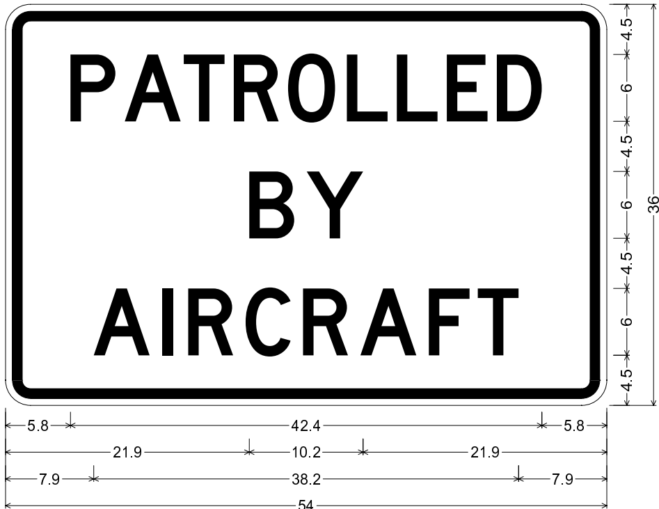
RNV19-1_54x36; 2.3" Radius, 0.9" Border, 0.6" Indent, Black on White; "PATROLLED" D 75% spacing; "BY" D; "AIRCRAFT" D;
