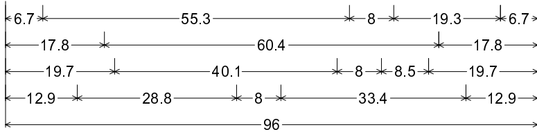
RNV28-1_96x66; 6.0" Radius, 1.5" Border, 1.3" Indent, Black on White; "PENALTIES FOR" D; "VIOLATIONS" D; "DOUBLE IN" D; "WORK ZONES" D;
