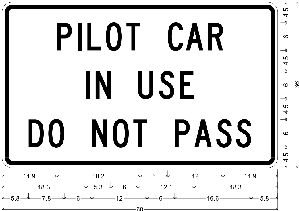
RNV30-1_60x36; 2.3" Radius, 0.9" Border, 0.6" Indent, Black on White; "PILOT CAR" C; "IN USE" C; "DO NOT PASS" C;
