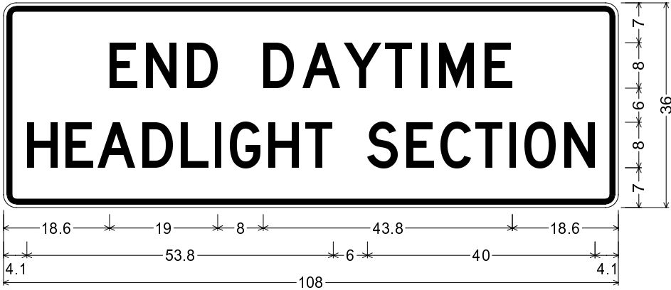
RNV8-2_108x36; 2.3" Radius, 0.9" Border, 0.6" Indent, Black on White; "END DAYTIME" D; "HEADLIGHT SECTION" D 75% spacing;
