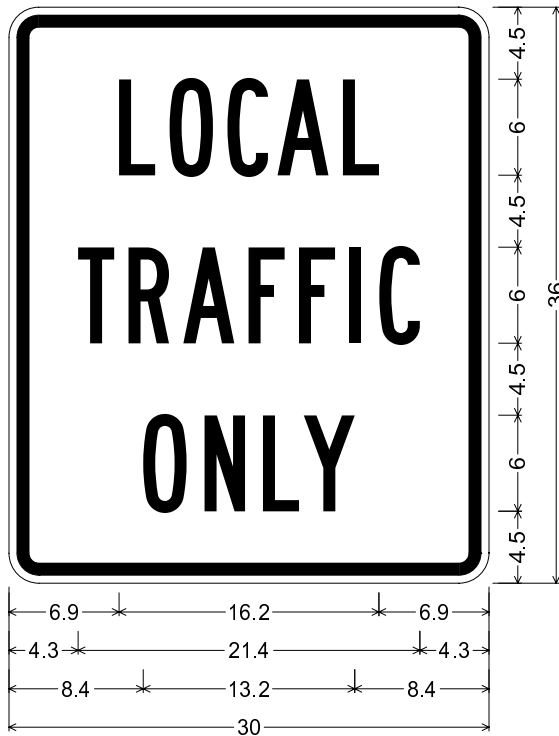
RNV24-1_30x36; 1.9" Radius, 0.8" Border, 0.5" Indent, Black on White; "LOCAL" B; "TRAFFIC" B; "ONLY" B;
