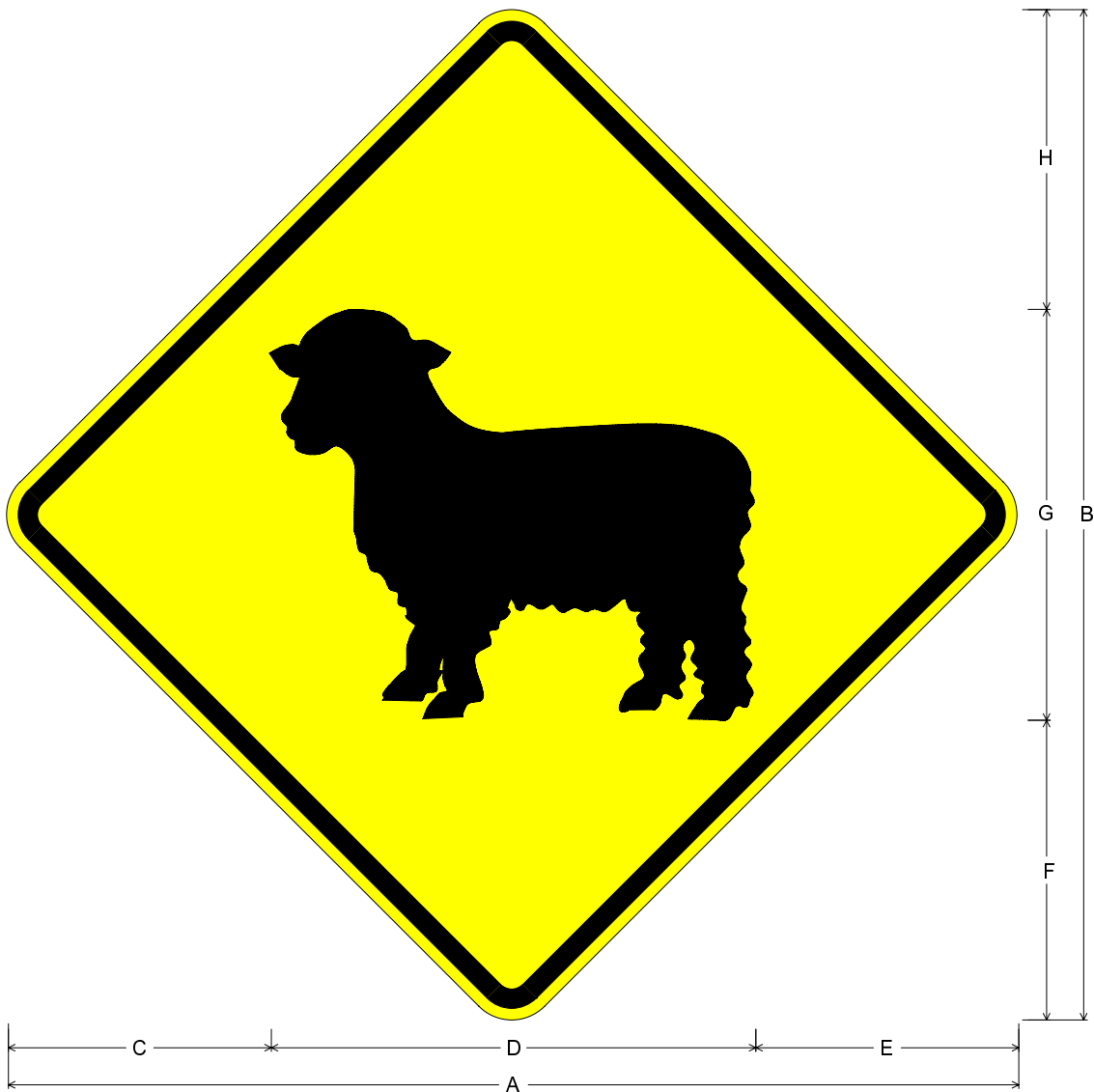
WNV15-7, Black on Yellow;
