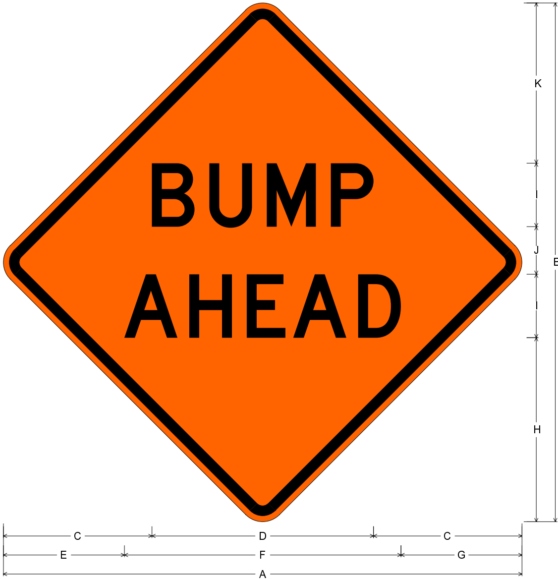
WNV23-1, Black on Orange; [BUMP] D; [AHEAD] D;
