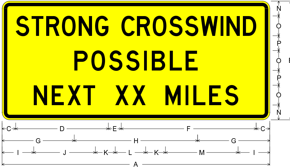
WNV5-1, Black on Yellow; [STRONG CROSSWIND]; [POSSIBLE]; [NEXT XX MILES] ;
