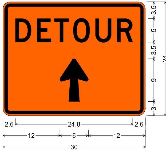
WNV20-1_30x24; 1.5" Radius, 0.6" Border, 0.4" Indent, Black on Orange; "DETOUR" D; Arrow Custom - 9.0" 90°;
