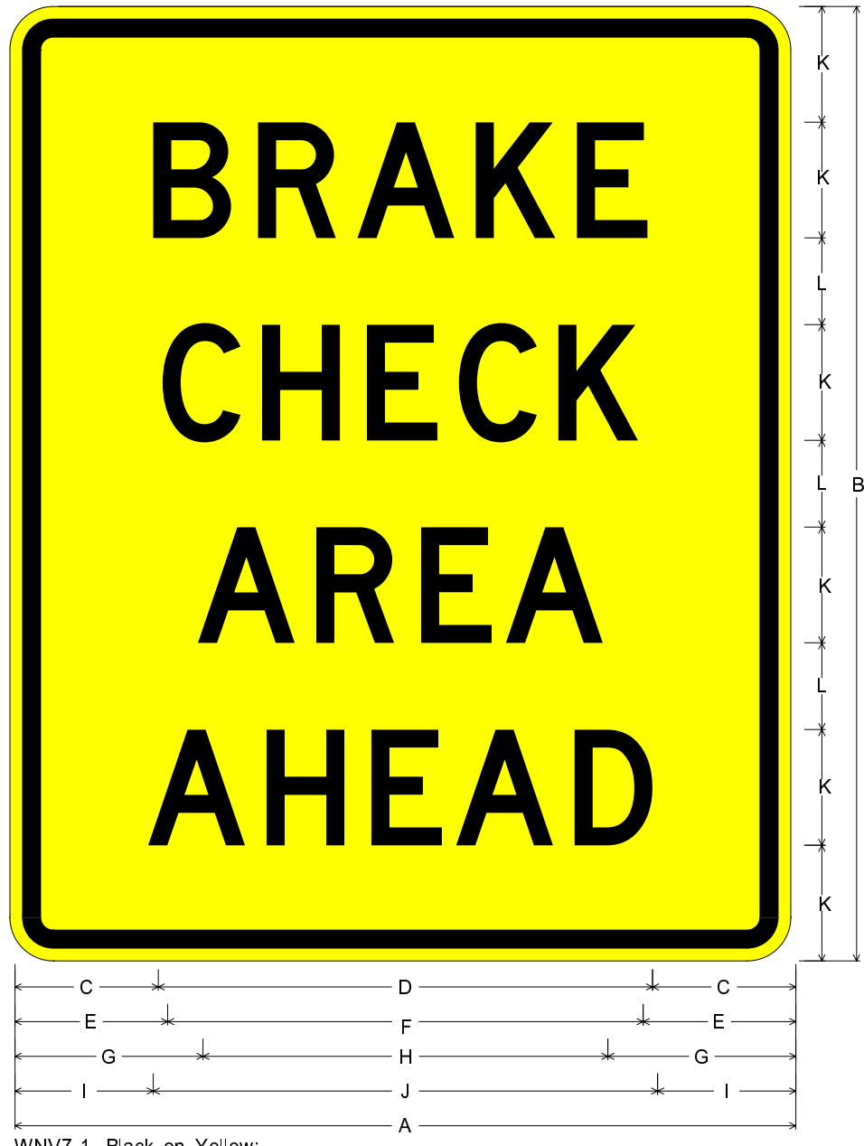
WNV7-1, Black on Yellow; [BRAKE] D; [CHECK] D; [AREA] D; [AHEAD] D;
