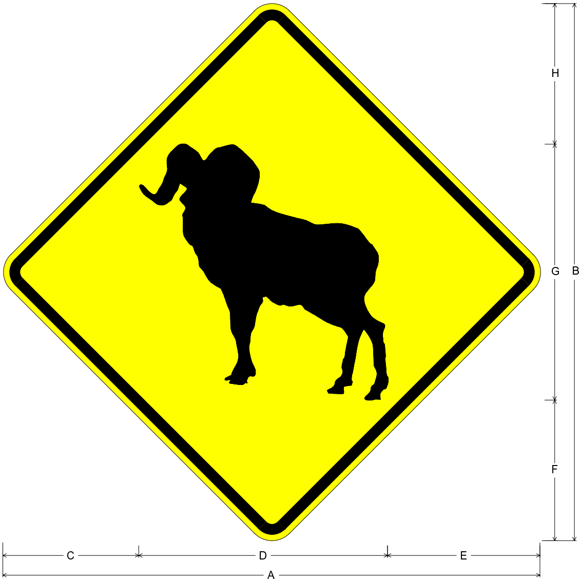
WNV15-6, Black on Yellow;
