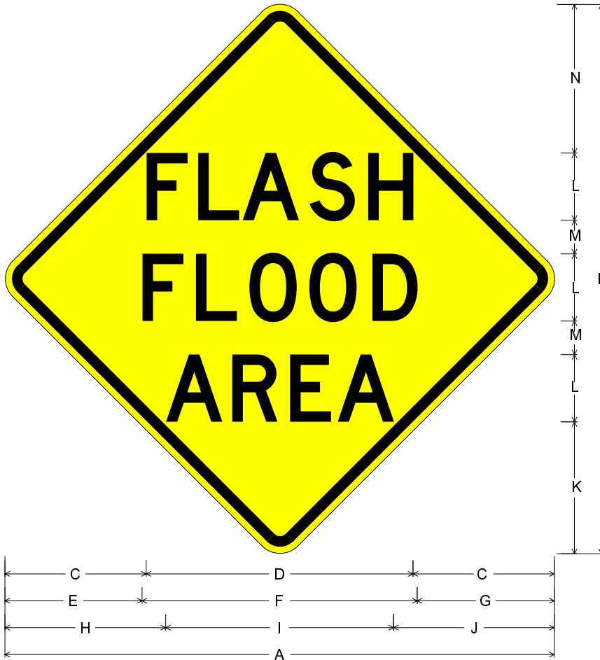
WNV11-1, Black on Yellow; [FLASH] D; [FLOOD] D; [AREA] D;
