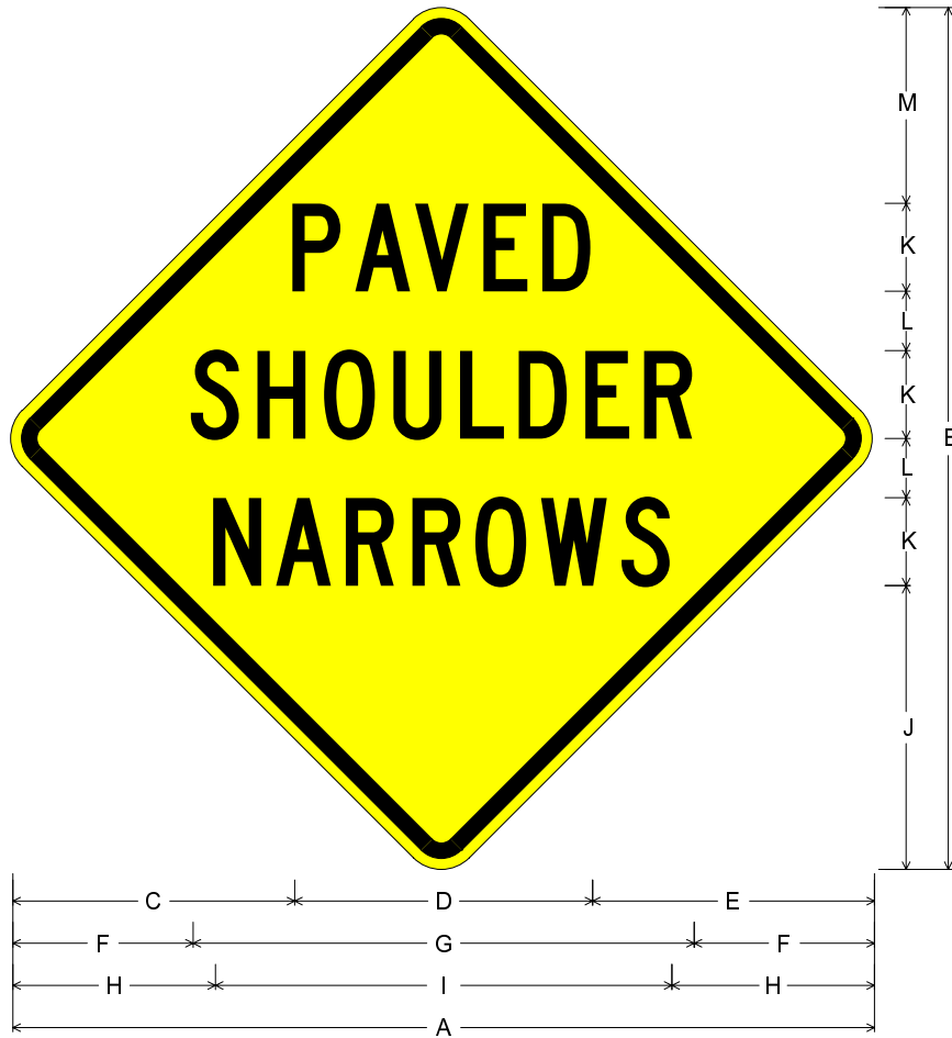
WNV9-1, Black on Yellow; [PAVED] C; [SHOULDER] C; [NARROWS] C;
