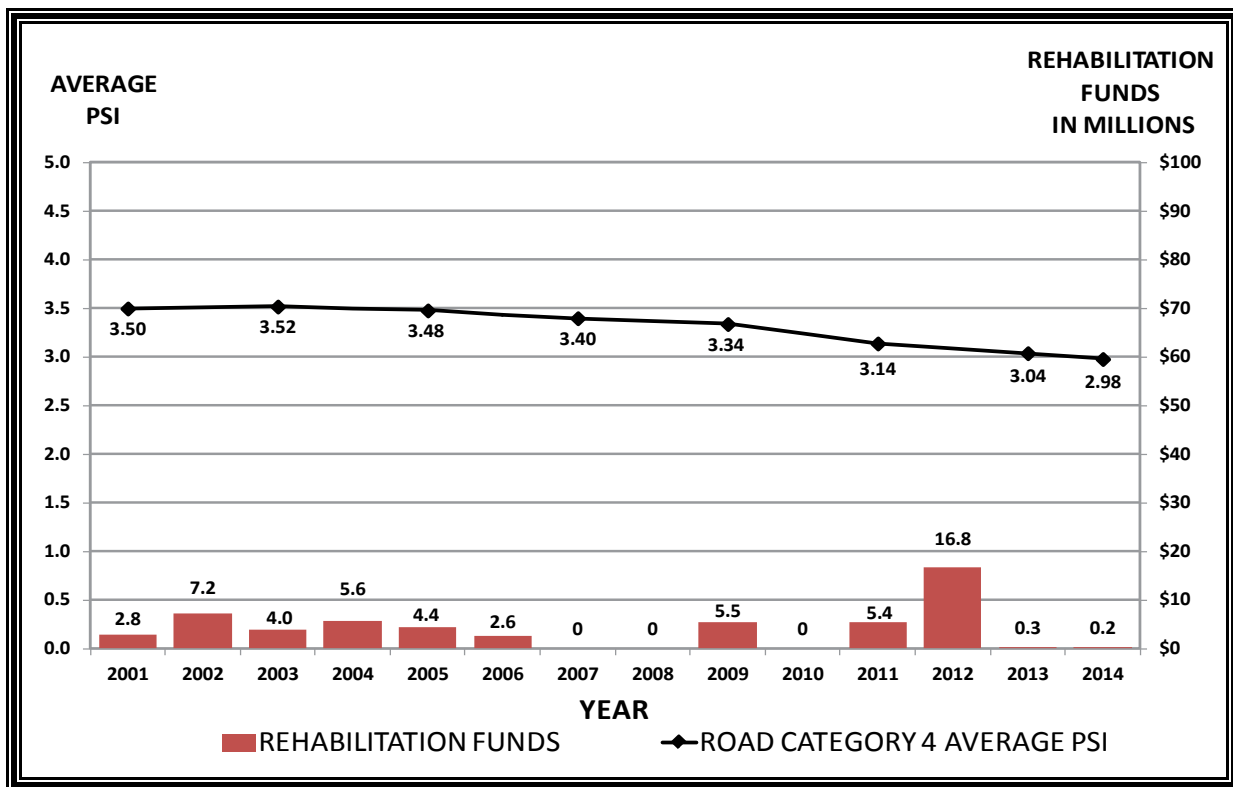
FIGURE 19. Average PSI and Expenditures for Road Category 4
