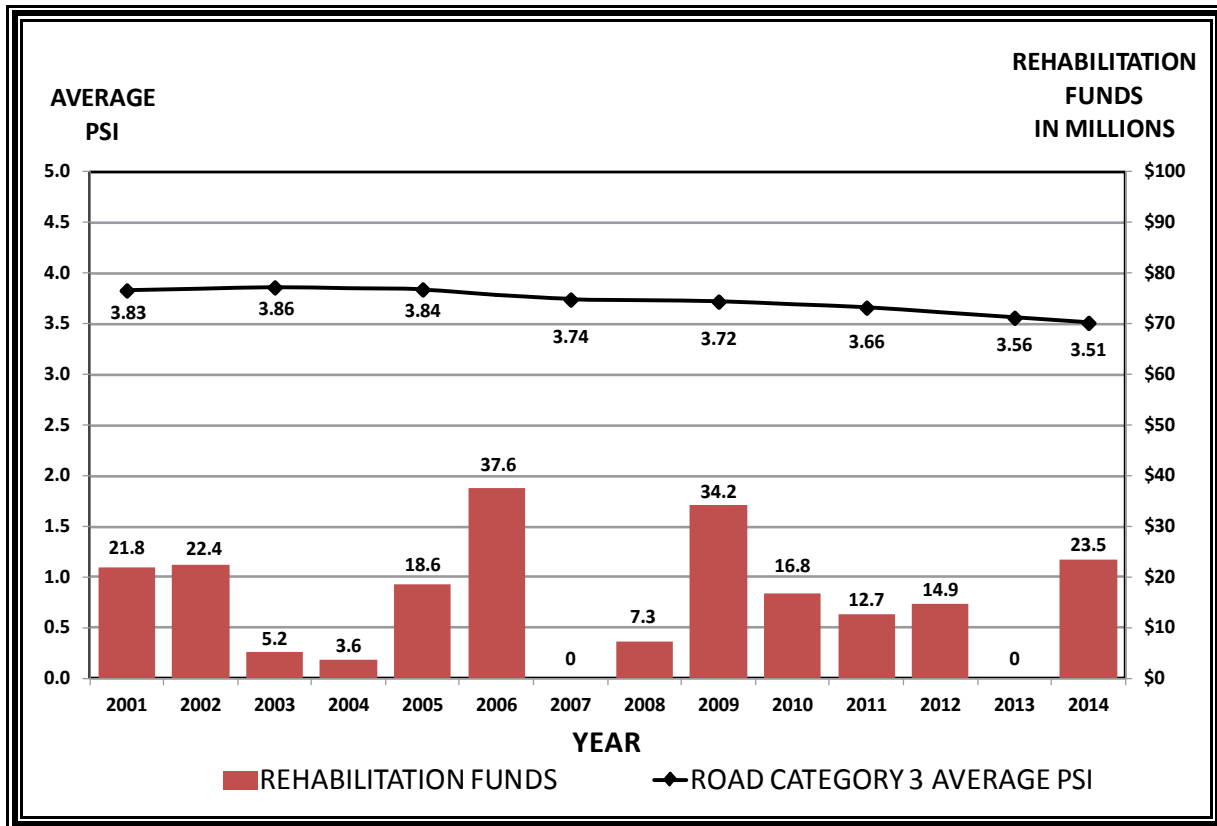
FIGURE 18. Average PSI and Expenditures for Road Category 3
