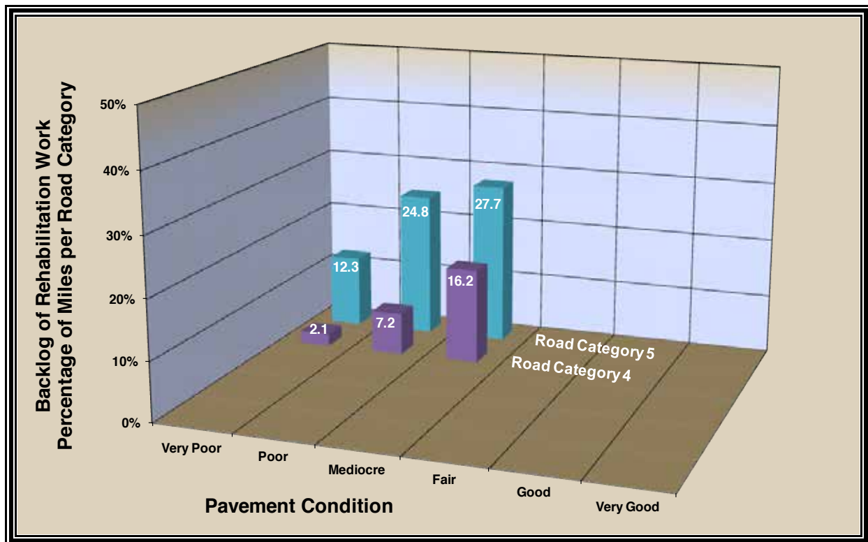
FIGURE 23. Backlog in Percentage of Miles per Road Category
