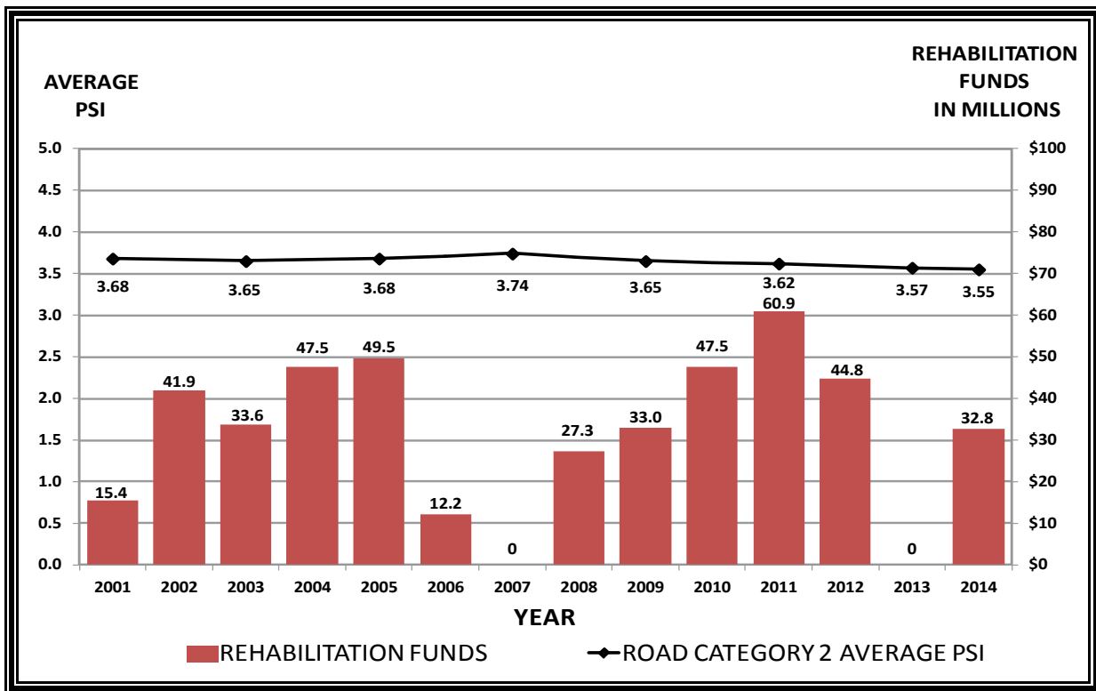
FIGURE 17. Average PSI and Expenditures for Road Category 2
