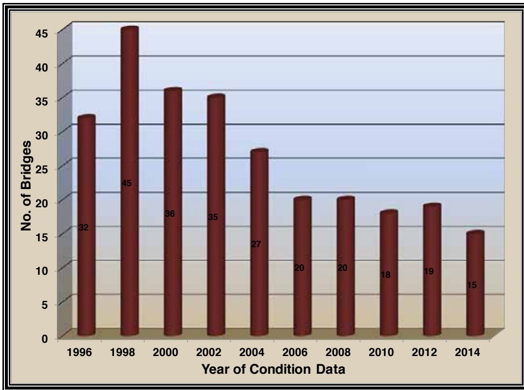
FIGURE 30. Structurally Deficient NDOT Bridges over Time
