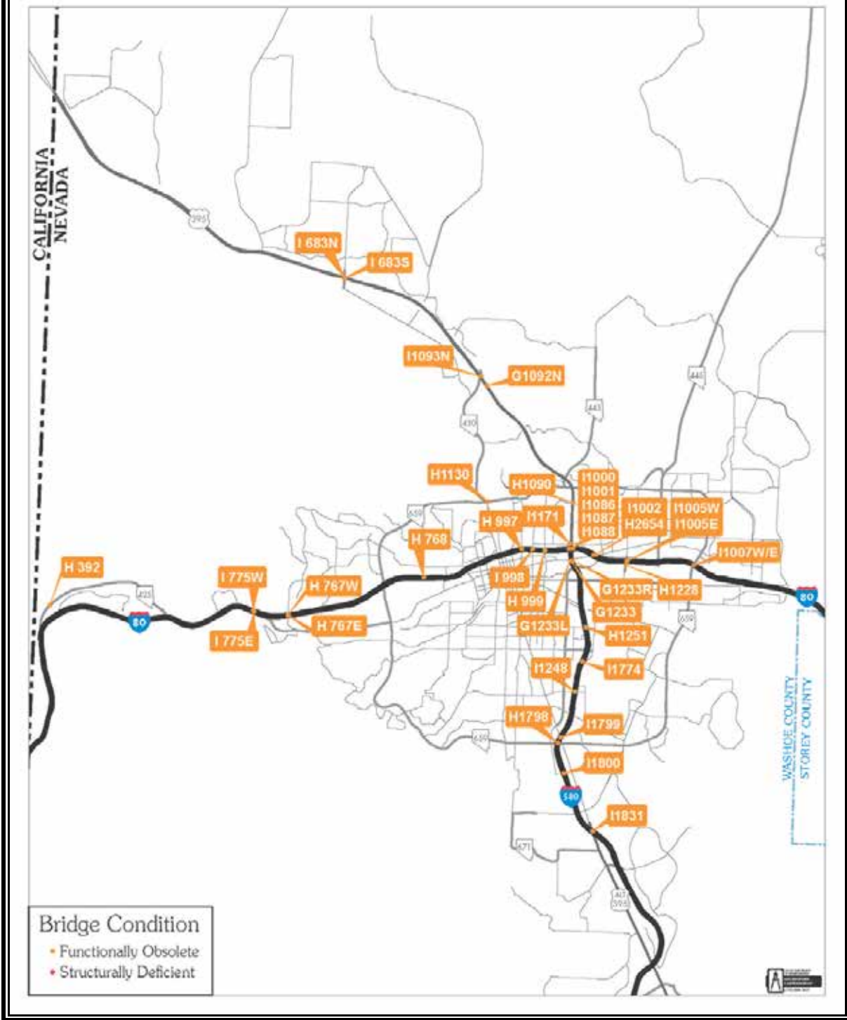
FIGURE 26C. Locations of Structurally Deficient and Functionally Obsolete Bridges
