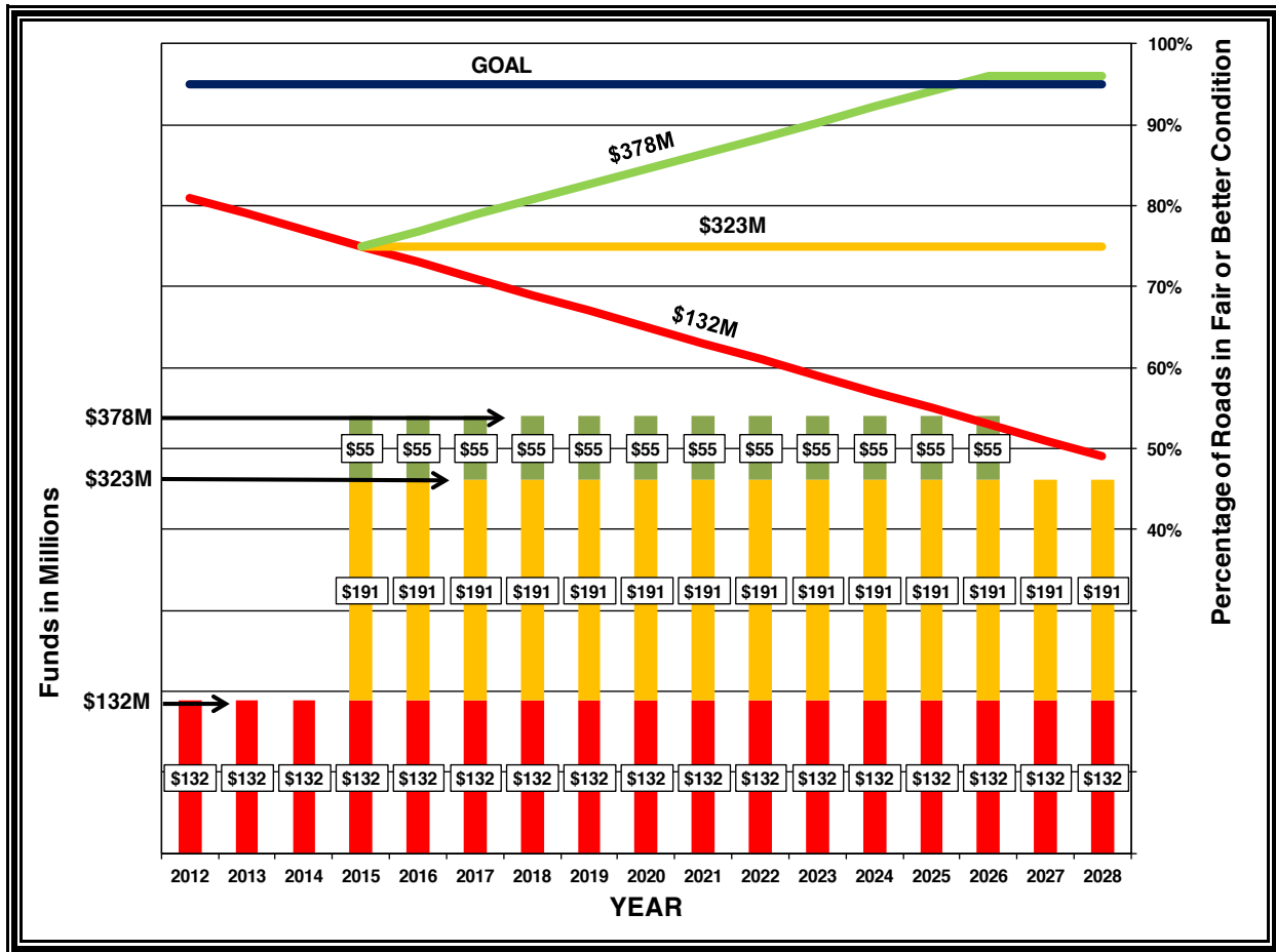
FIGURE 24. Future State-maintained Roadway Network Funding Options
