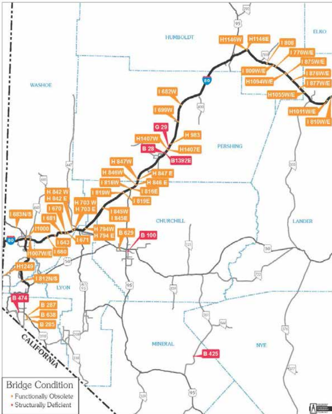
FIGURE 26D. Locations of Structurally Deficient and Functionally Obsolete Bridges
