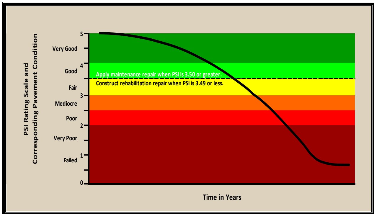
FIGURE 3. Timing for Repair Strategies Based on PSI Rating System
