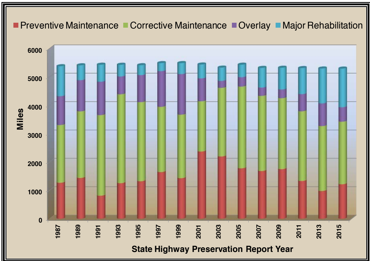
FIGURE 21. Change in Pavement Condition Over Time Based on Repair Strategies
