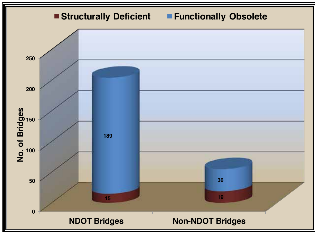
FIGURE 25. Substandard Bridges
