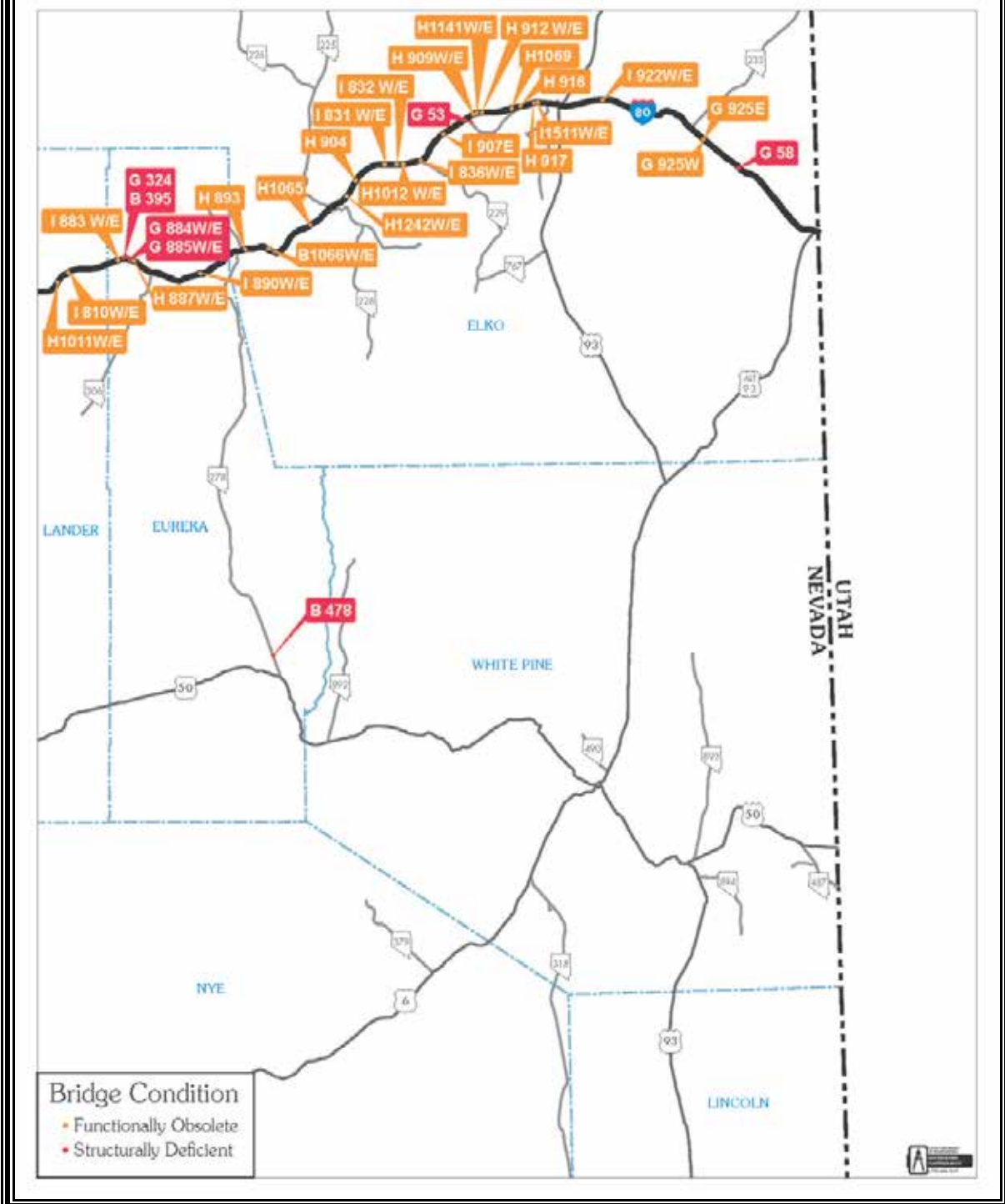
FIGURE 26E. Locations of Structurally Deficient and Functionally Obsolete Bridges
