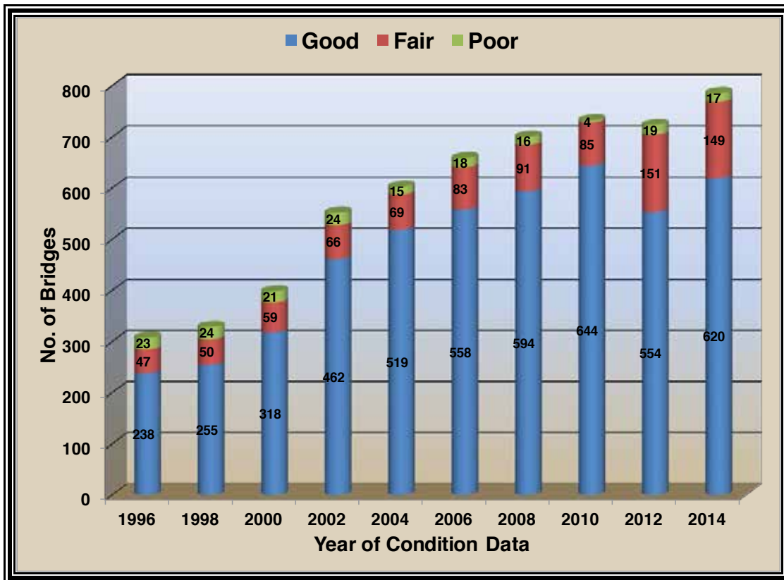
FIGURE 31. Non-NDOT Bridge Conditions over Time
