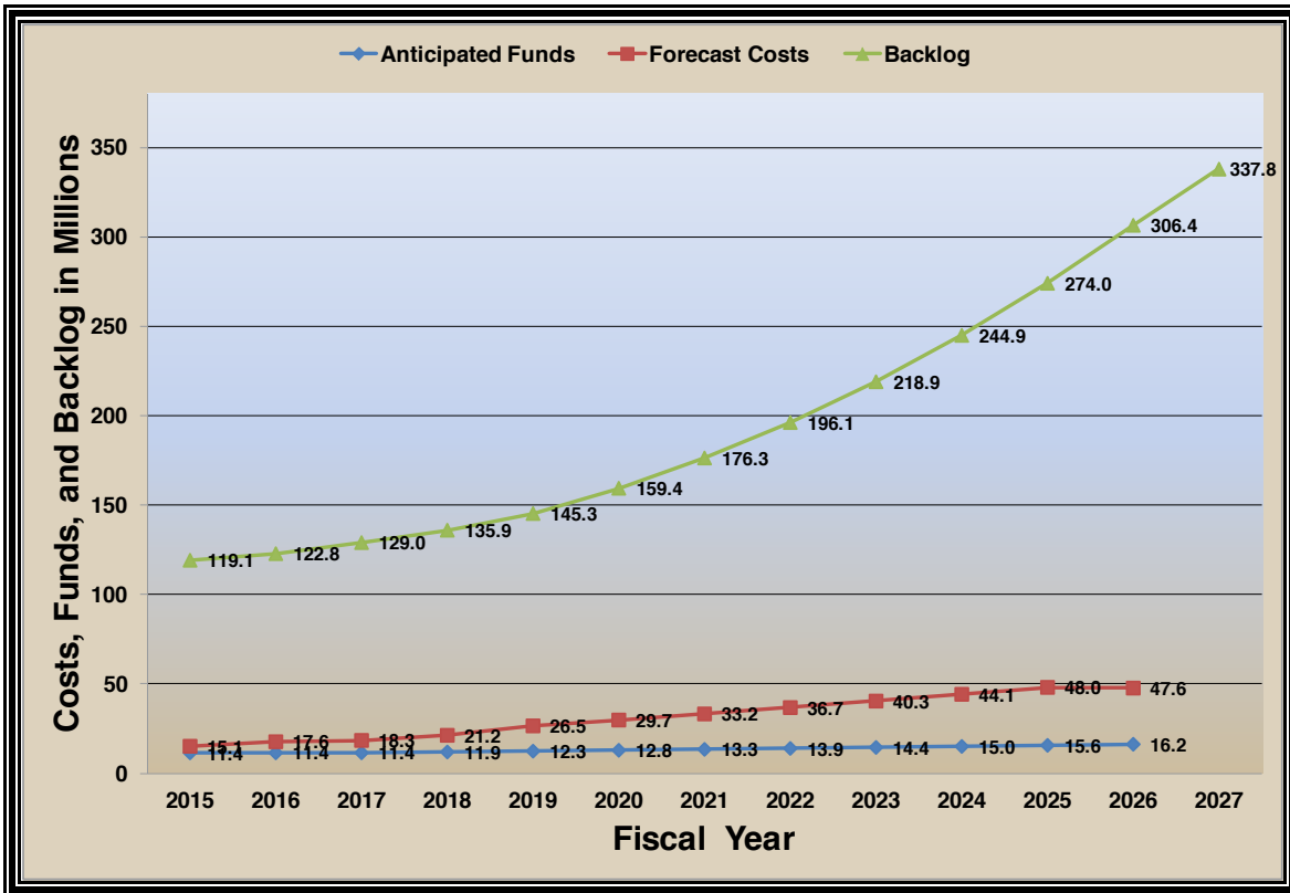
FIGURE 34. Anticipated Costs, Funds and Backlog of Bridge Preservation Work
