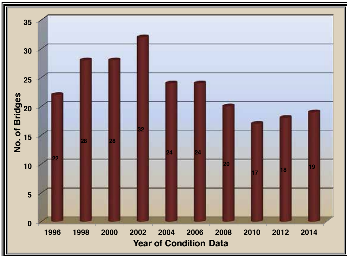
FIGURE 32. Structurally Deficient Non-NDOT Bridges over Time
