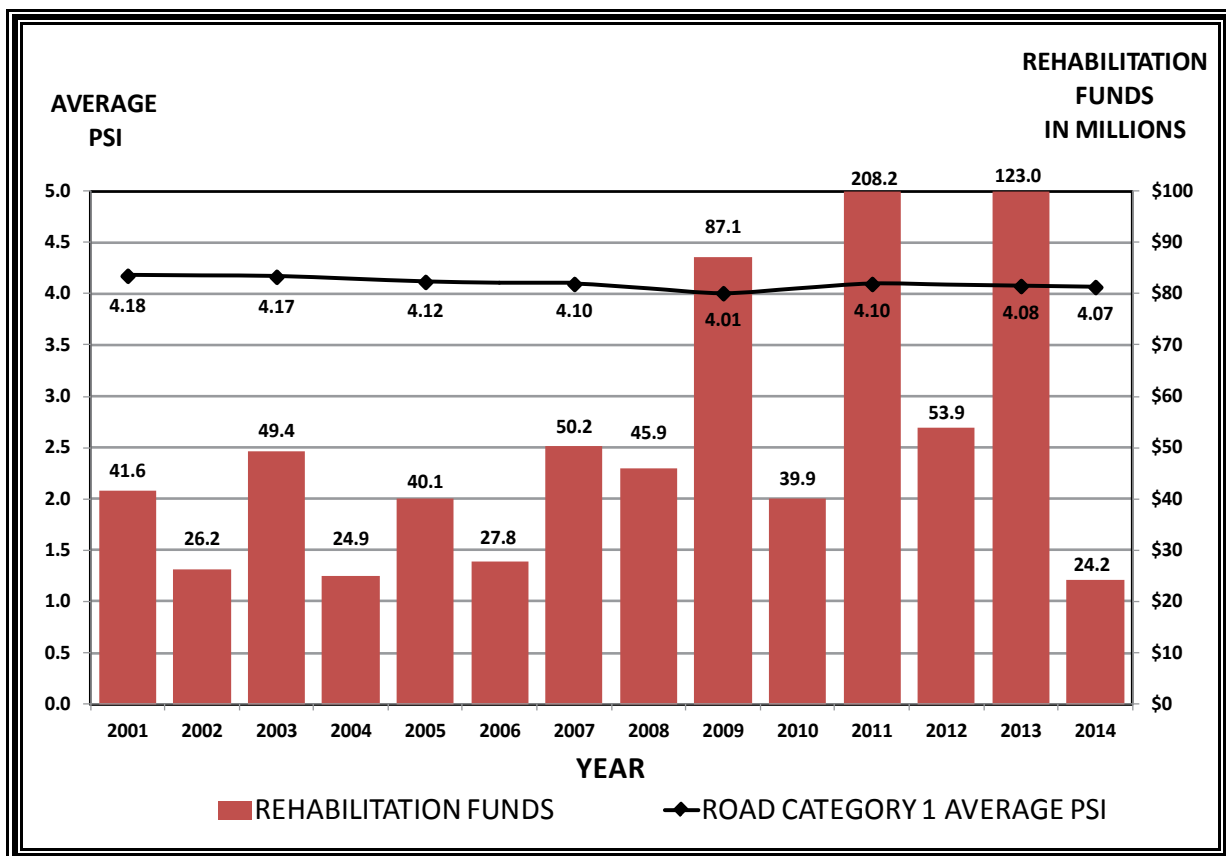
FIGURE 16. Average PSI and Expenditures for Road Category 1
