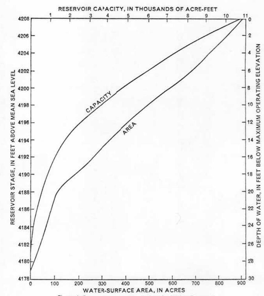
Figure 4.—Stage-area-capacity relations for Weber Reservoir
