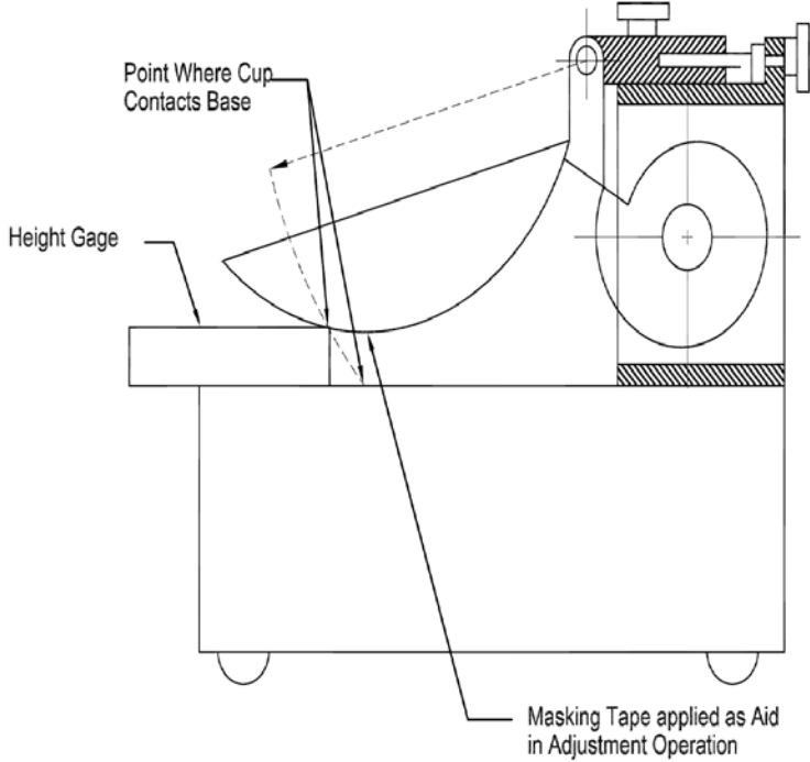
Figure 2 —Calibration for Height of Drop
