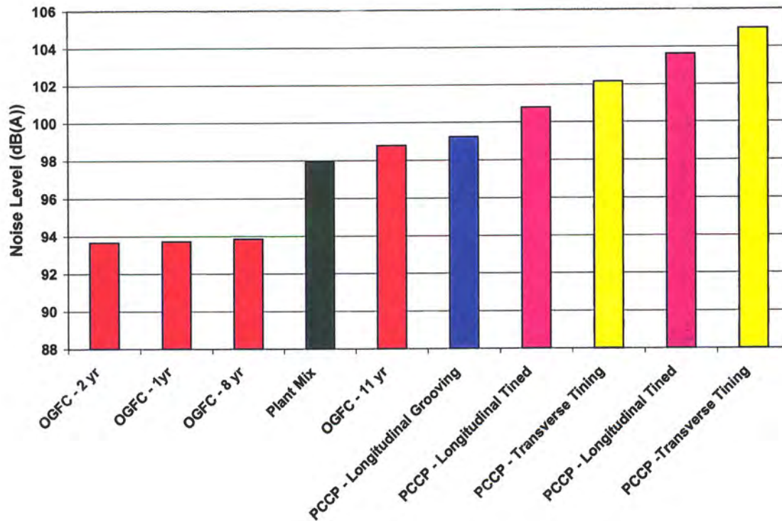
Figure 8 – Chart Comparing Pavements Tested
