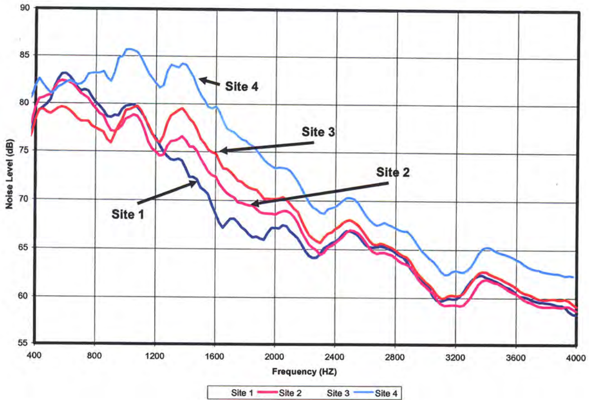
Figure 9 –Frequency Spectrum for the OGFC Surfaces
