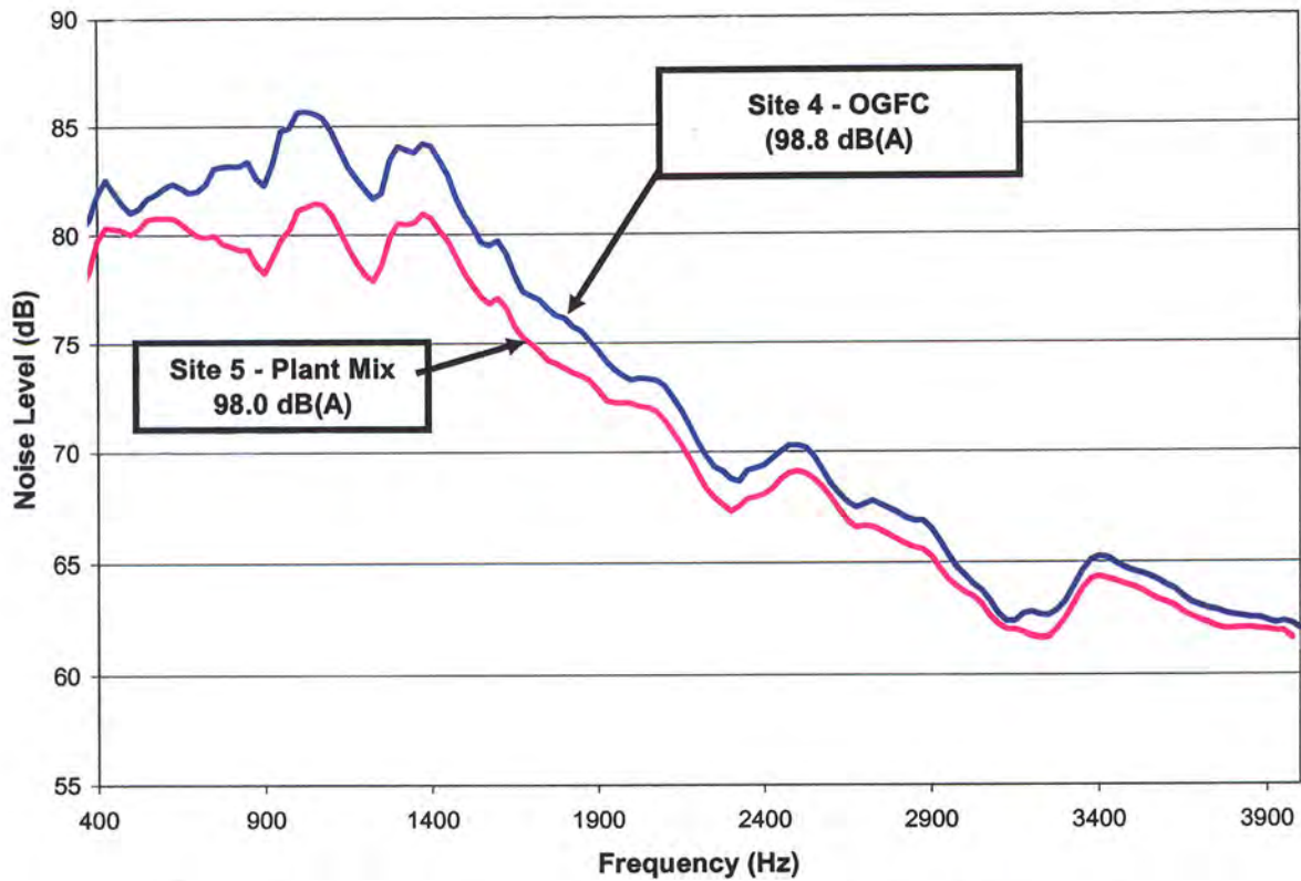
Figure 12 – Comparison of Frequency Spectrums for Sites 4 and 5
