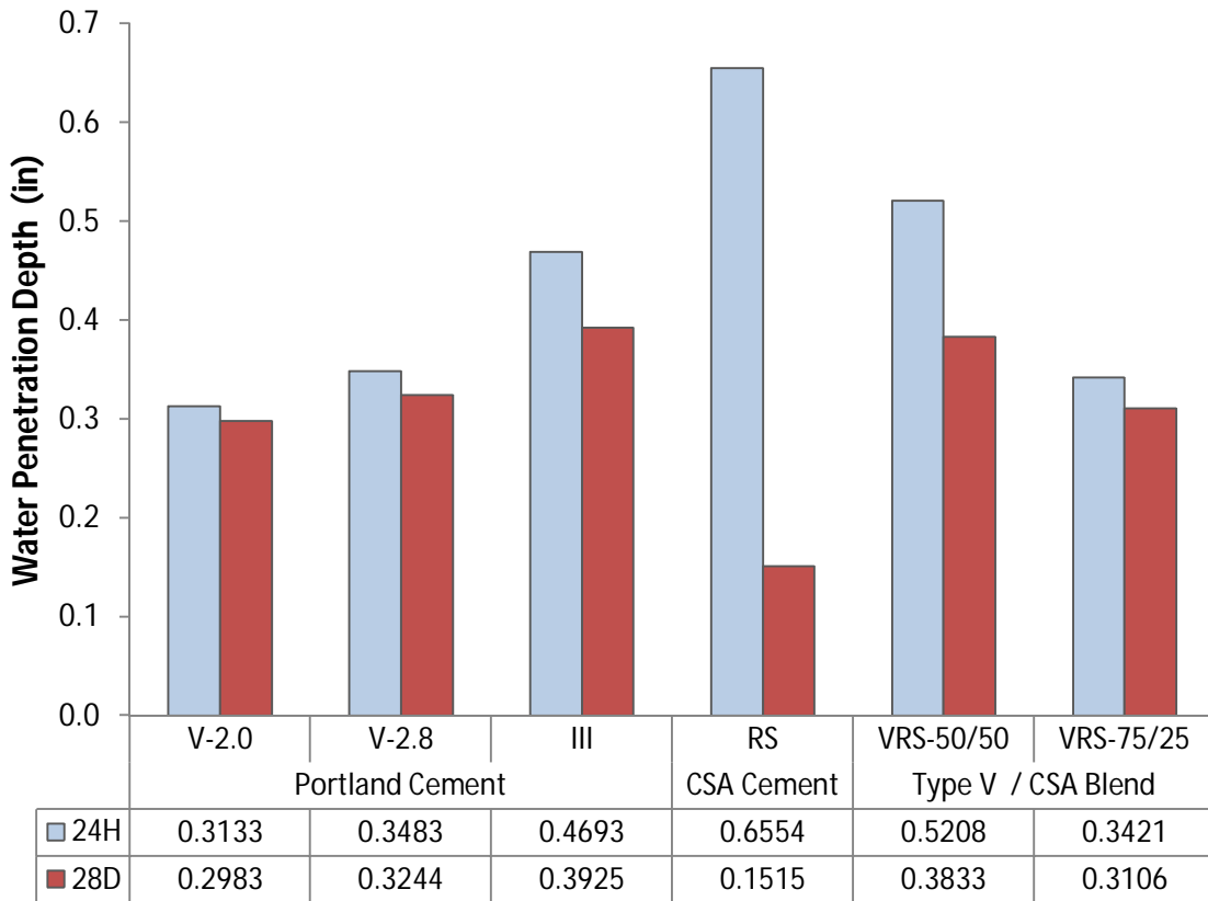
Figure 7-7: Water Penetration Depth of Selected HES Concretes
