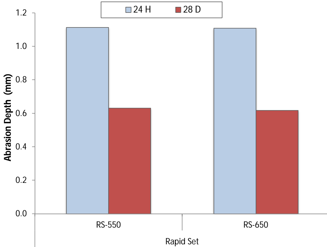
Figure 6-16: Abrasion Depth of Rapid Set HES Concretes
