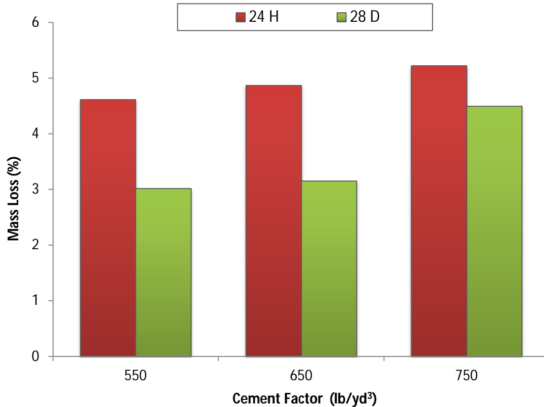
Figure 5-15: Ultimate Mass Loss of Type III-HES Concretes Subjected to 25 Freezing and Thawing Cycles
