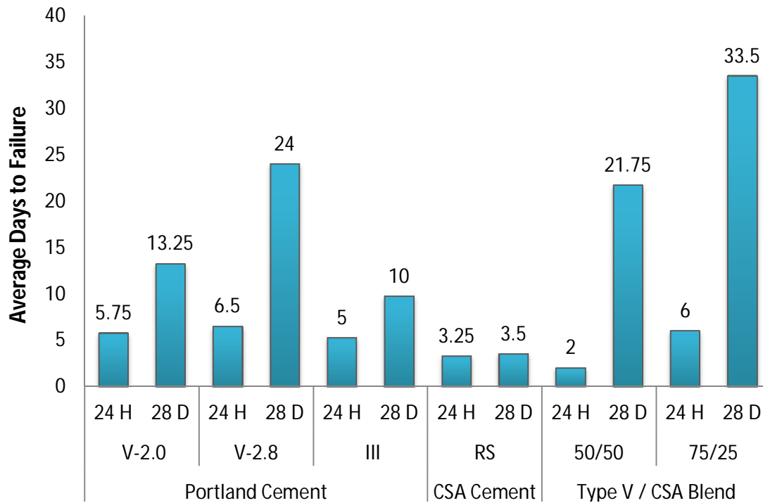
Figure 7-10: Failure Time of HES Concretes in Corrosion Test
