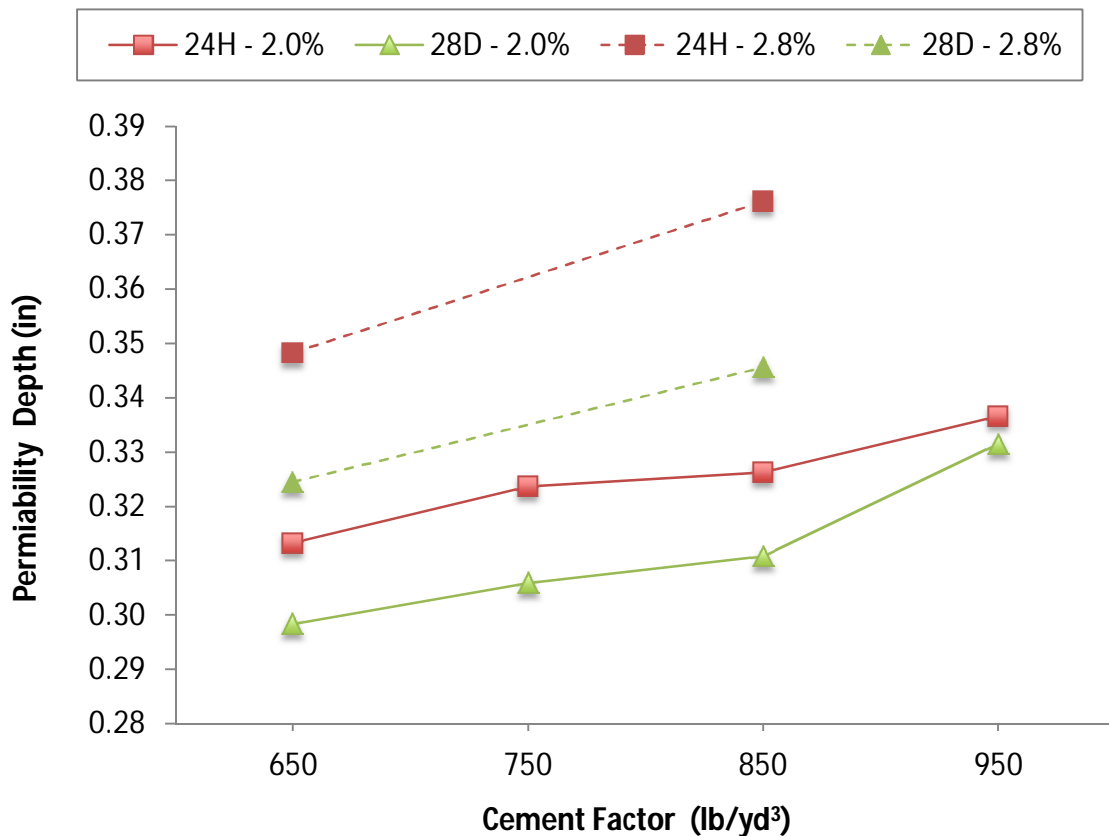
Figure 4-7: Water Penetration Depth of Type V-HES Concretes
