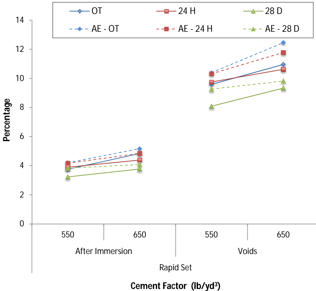
Figure 6-4: Absorption and Volume of Permeable Voids Rapid Set HES Concretes
