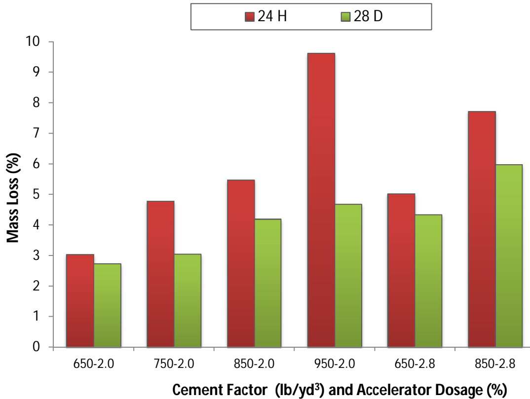
Figure 4-16: Ultimate Mass Loss of Type V-HES Concretes Subjected to 25 Freezing and Thawing Cycles
