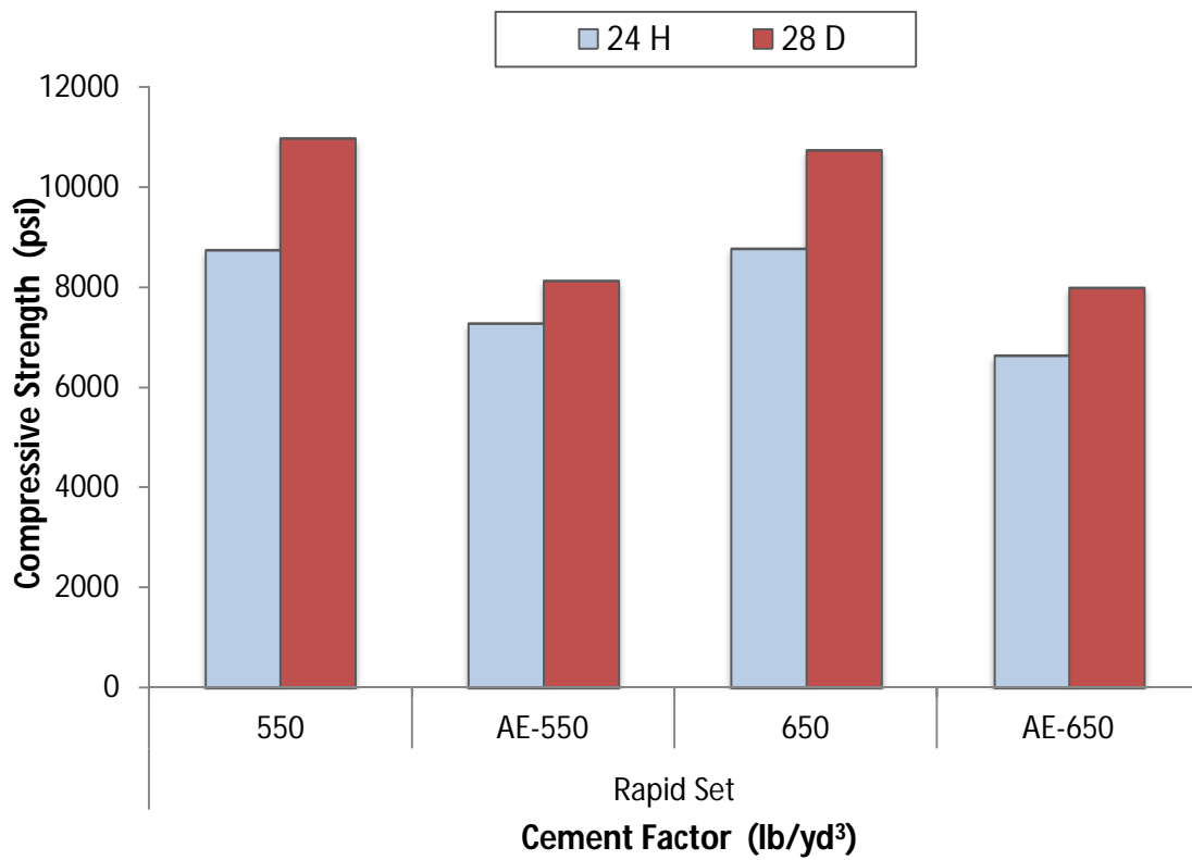
Figure 6-2: Compressive Strength Rapid Set HES Concretes at 24 Hrs and 28 Days
