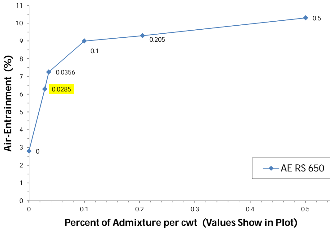
Figure 3-2: Air Content of Rapid Set concrete as a Function of Air-Entraining Admixture, Cement Factor 650 lb/yd 3
