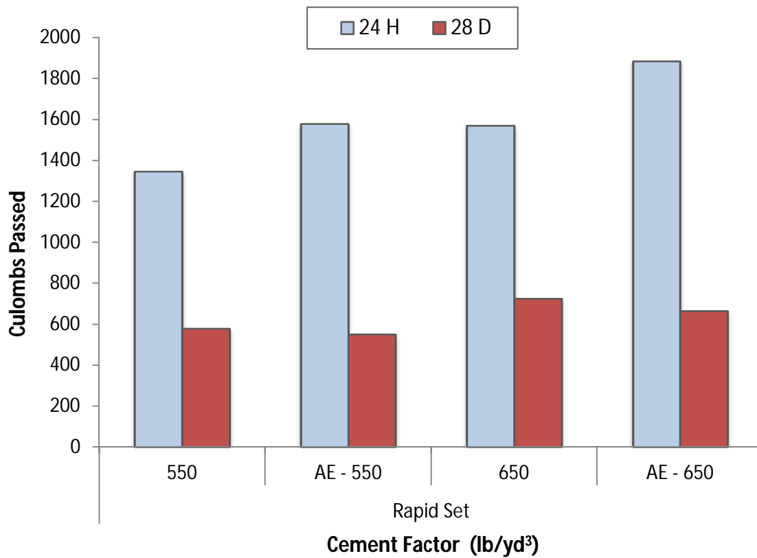
Figure 6-5: Passing Charge of Rapid Set HES Concretes
