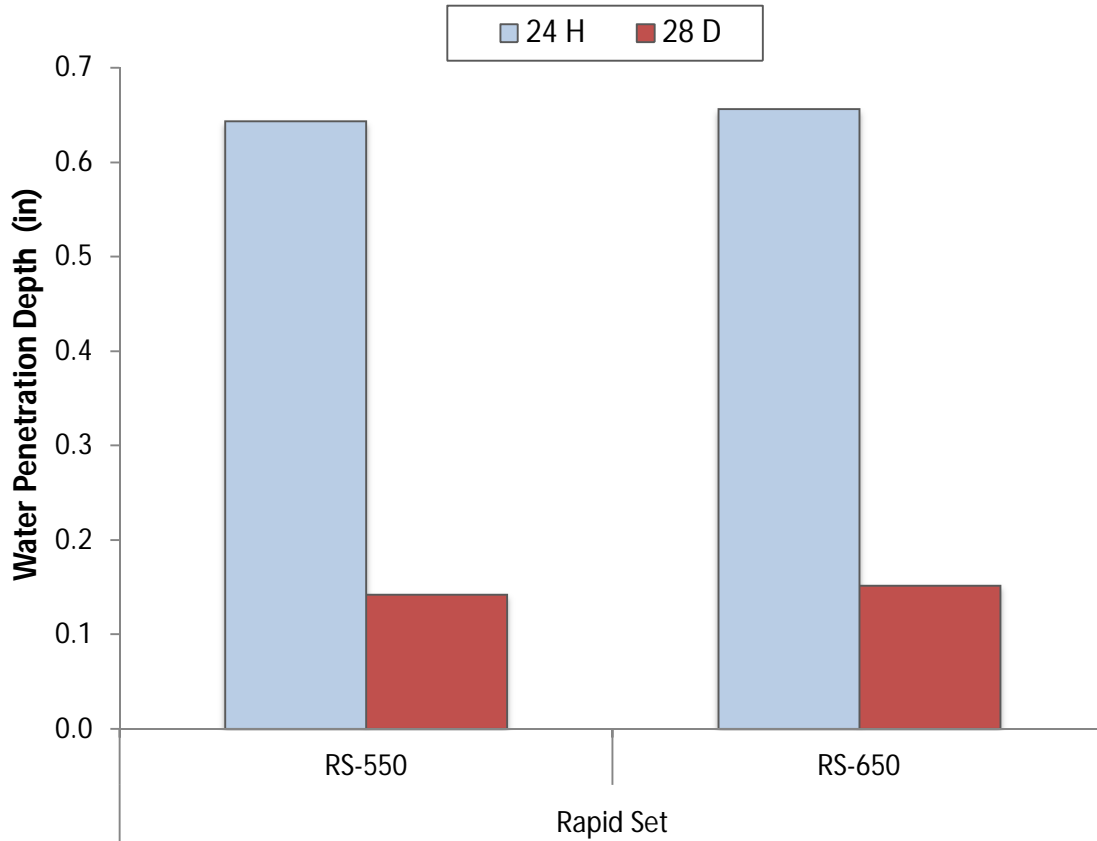
Figure 6-7: Water Penetration Depth of Rapid Set HES Concretes
