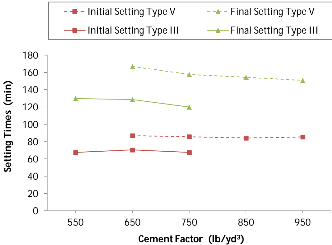
Figure 3-1: Initial and Final Setting Times for Type III and Type V
