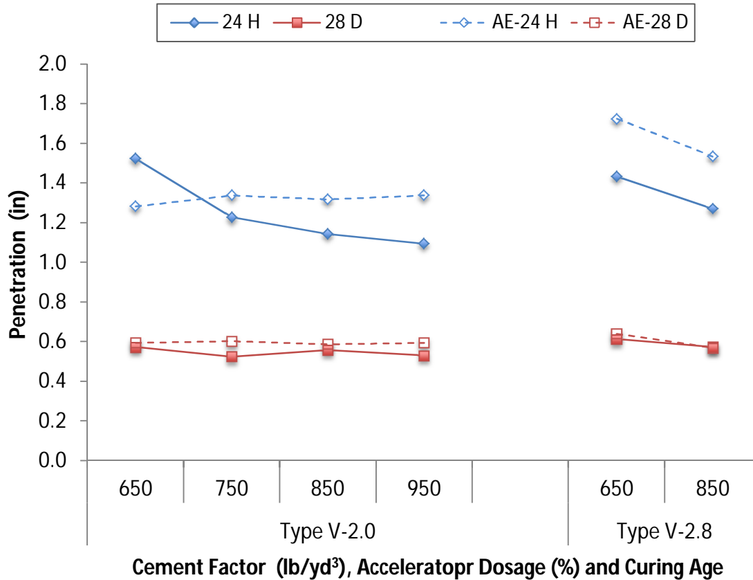
Figure 4-6: Chloride Penetration Depth of Type V-HES Concretes
