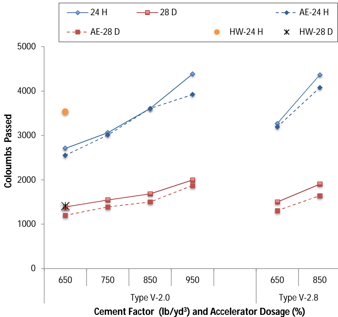
Figure 4-5: Passing Charges of Type V-HES Concretes
