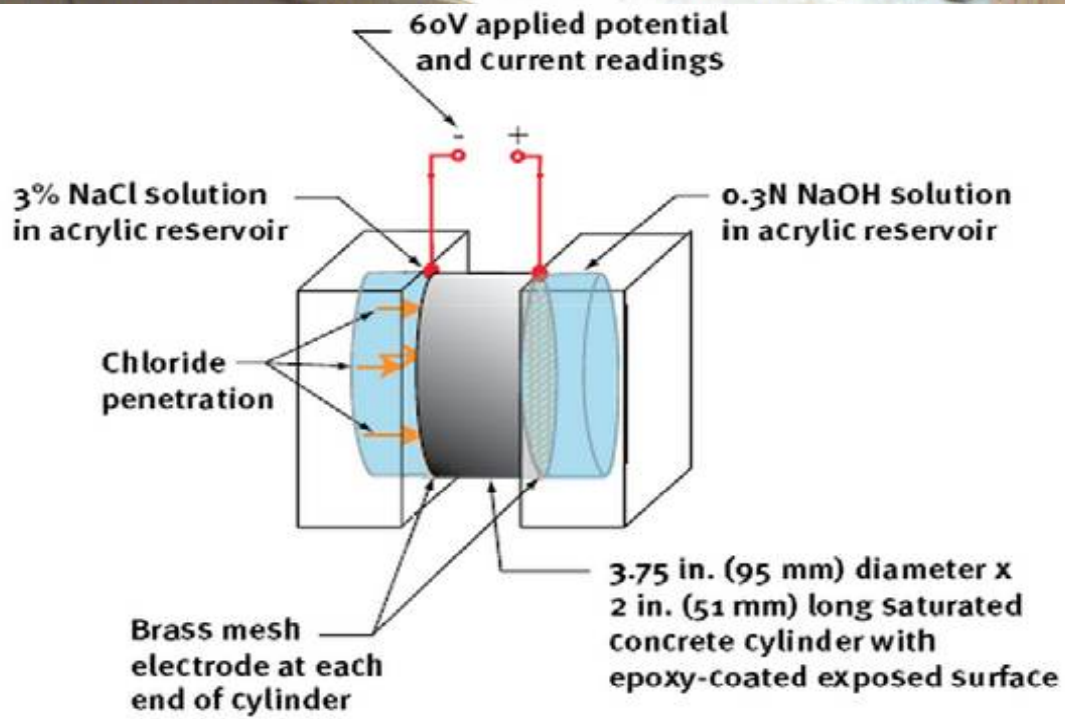
Figure 2-12: RCPT Set-Up and Schematic
