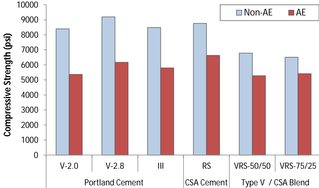
Figure 7-1: Compressive Strength of the Selected HES Concretes at 24 hrs
