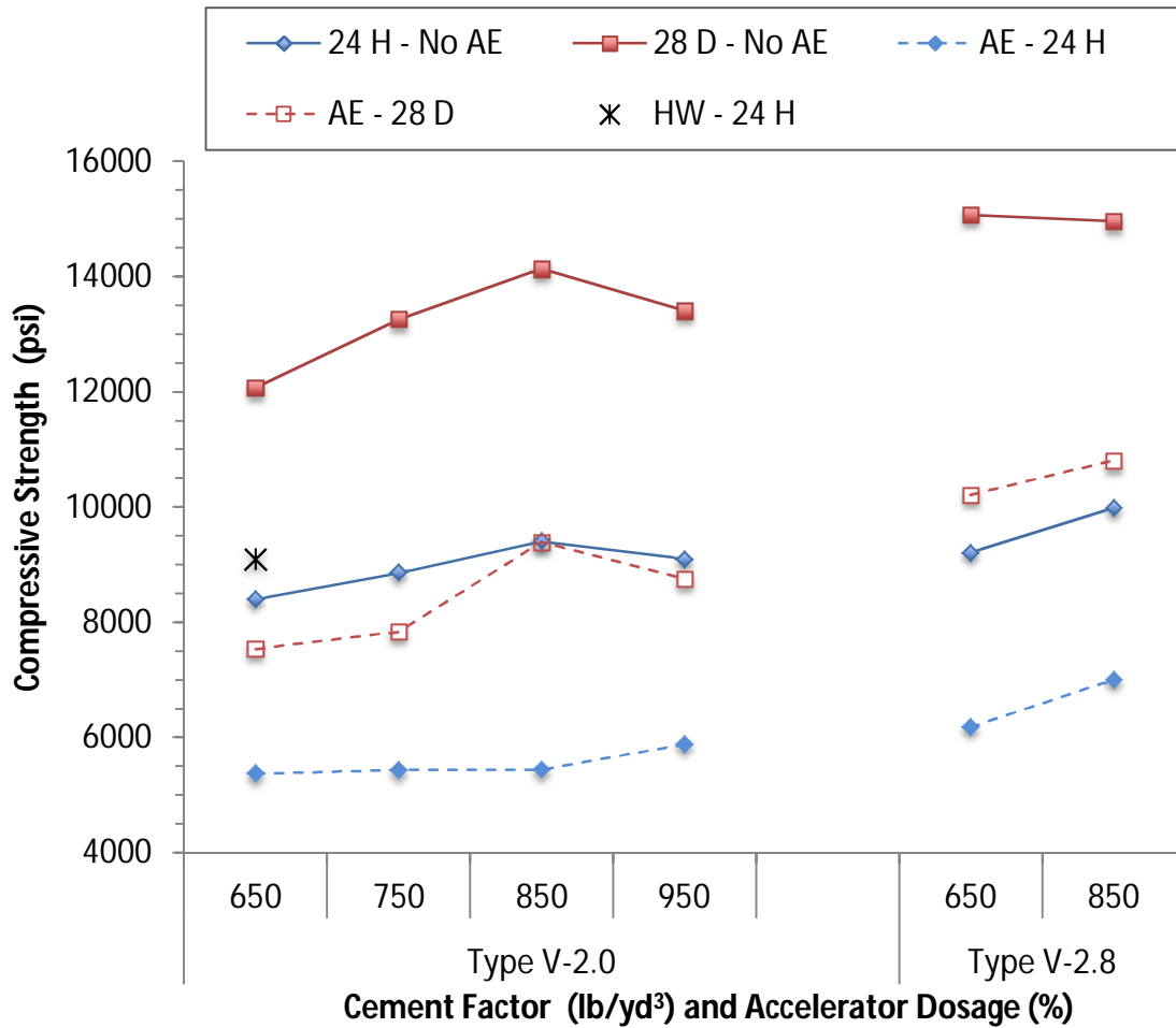
Figure 4-2: Compressive Strength of Type V-HES Concretes at 24 Hrs and 28 Days
