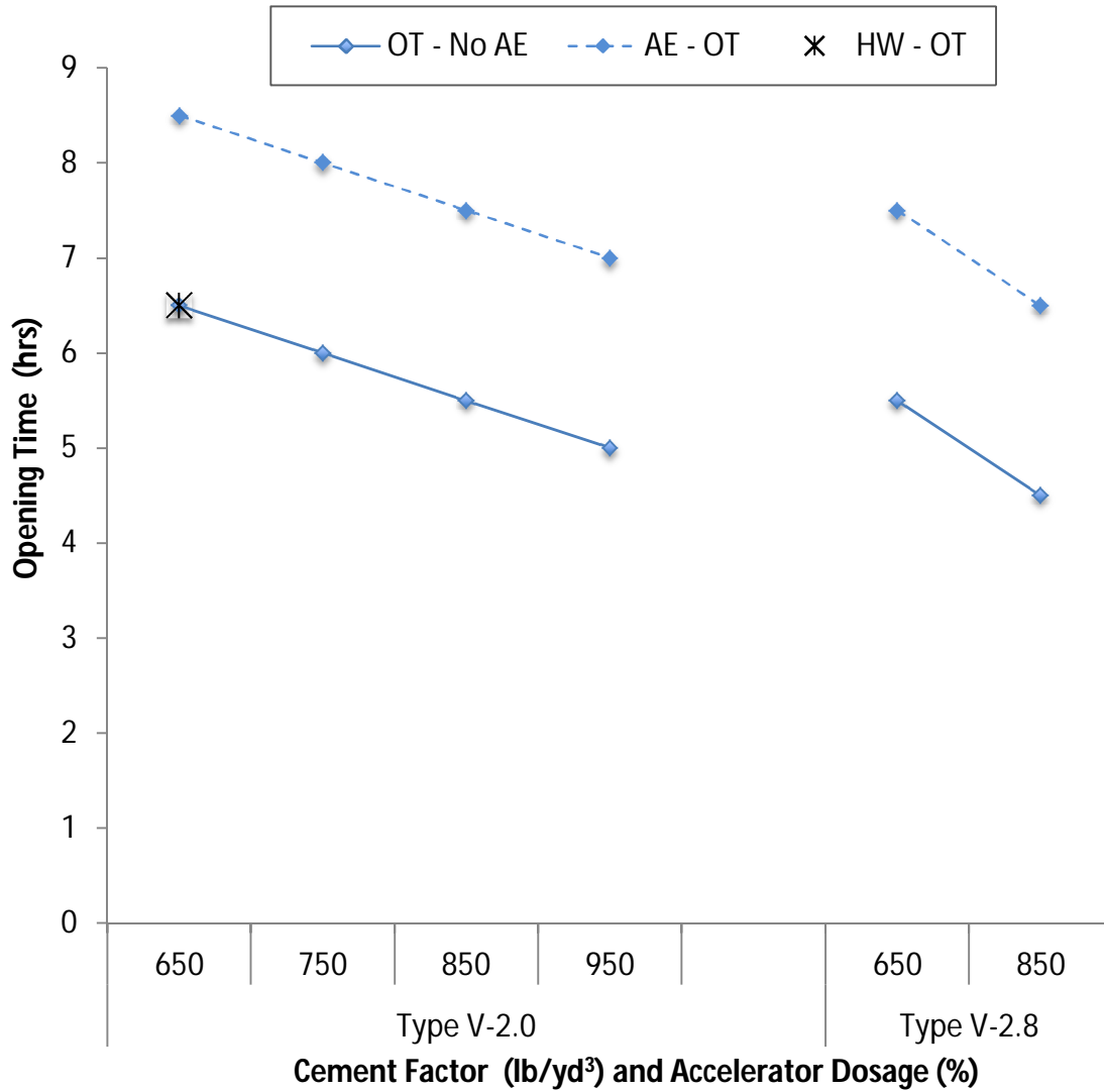
Figure 4-1: Opening Time of Type V-HES Concretes
