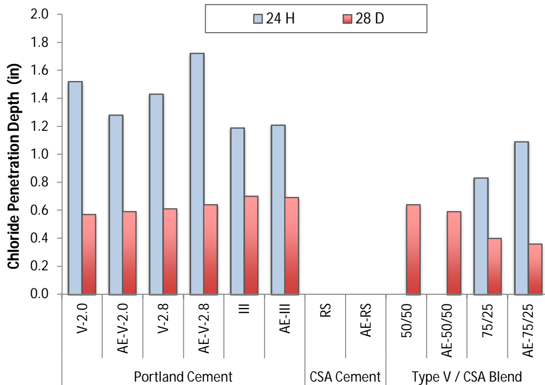
Figure 7-6: Chloride Penetration Depth of the Selected HES Concretes
