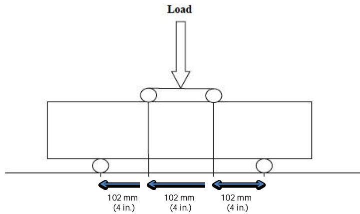
Figure 2-8: Flexure Schematic for 4-Point Loading (a.k.a. 1/3 Point Loading)
