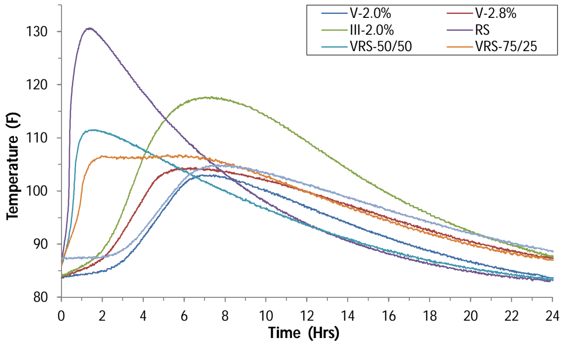
Figure 3-4: Typical Heat of Hydration Trends for Non-Air-Entrained HES Concretes (650 lb/yd 3 )
