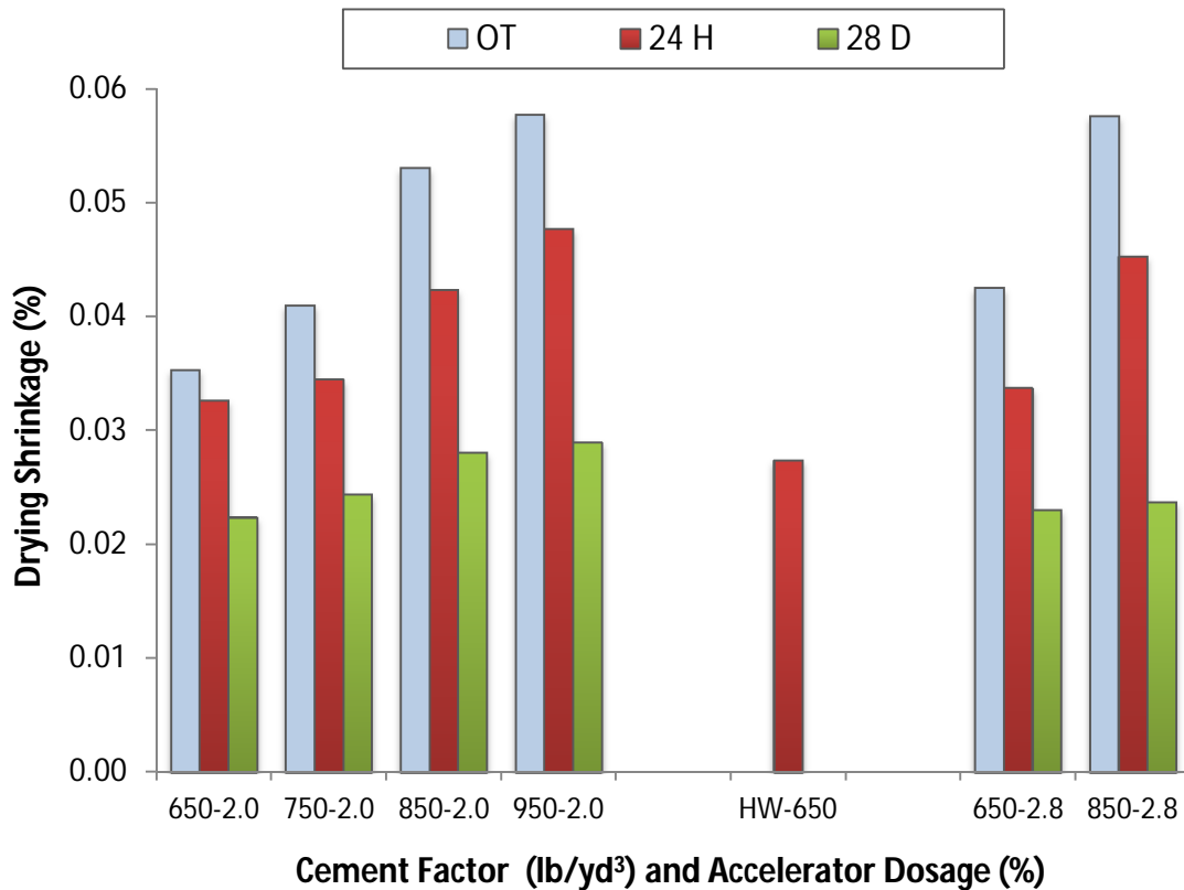
Figure 4-12: Drying Shrinkage of Type V-HES Concretes After 28 Days in Shrinkage Room
