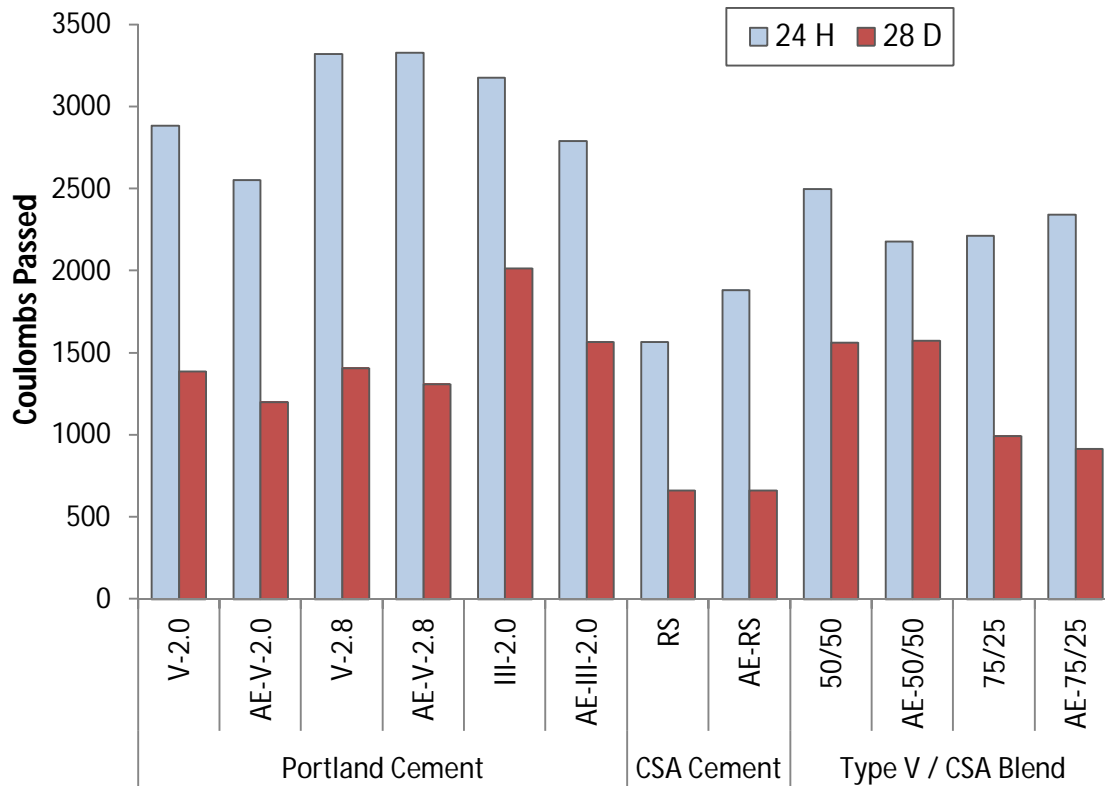
Figure 7-5: Passing Charges of the Selected HES Concretes
