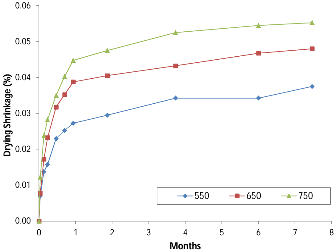
Figure 5-9: Drying Shrinkage of Type III-HES Concretes Transferred to Shrinkage Room at the Age of 24 Hrs
