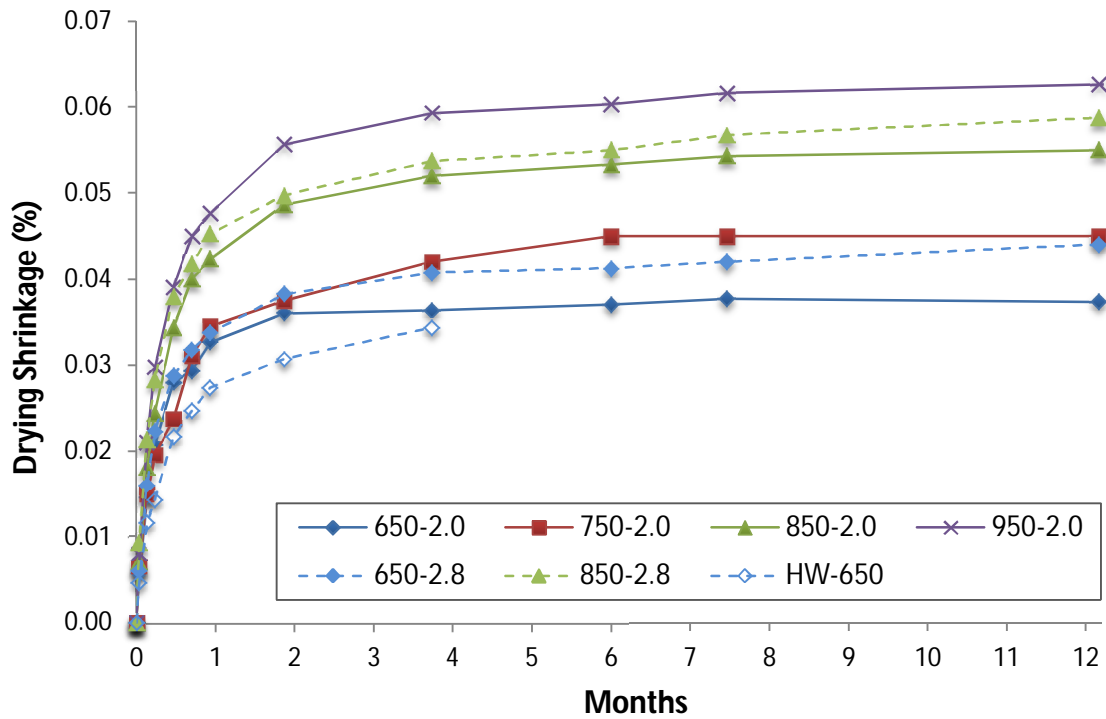
Figure 4-9: Drying Shrinkage of Type V-HES Concretes Transferred to Shrinkage Room at the Age of 24 Hrs
