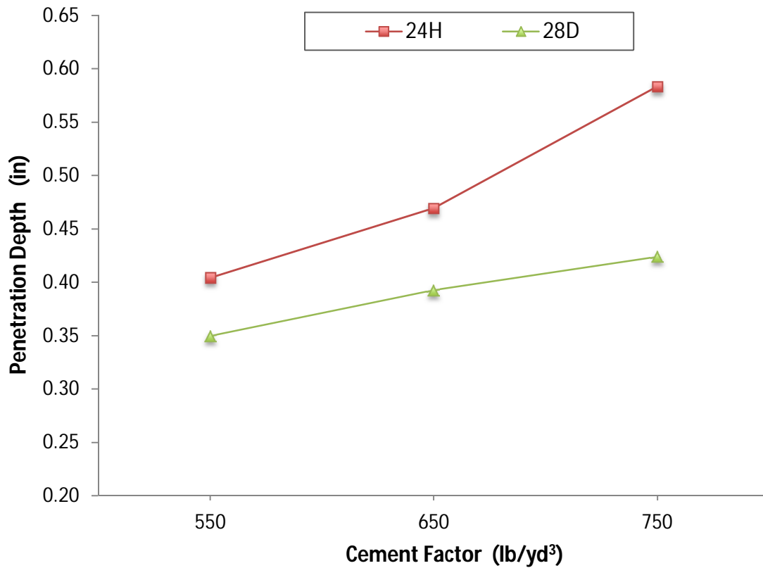
Figure 5-7: Water Penetration Depth of Type III-HES Concretes
