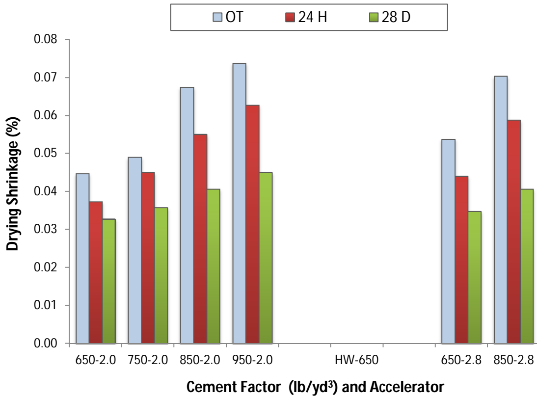
Figure 4-11: The Ultimate Shrinkage (1-Year) of Type V-HES Concretes
