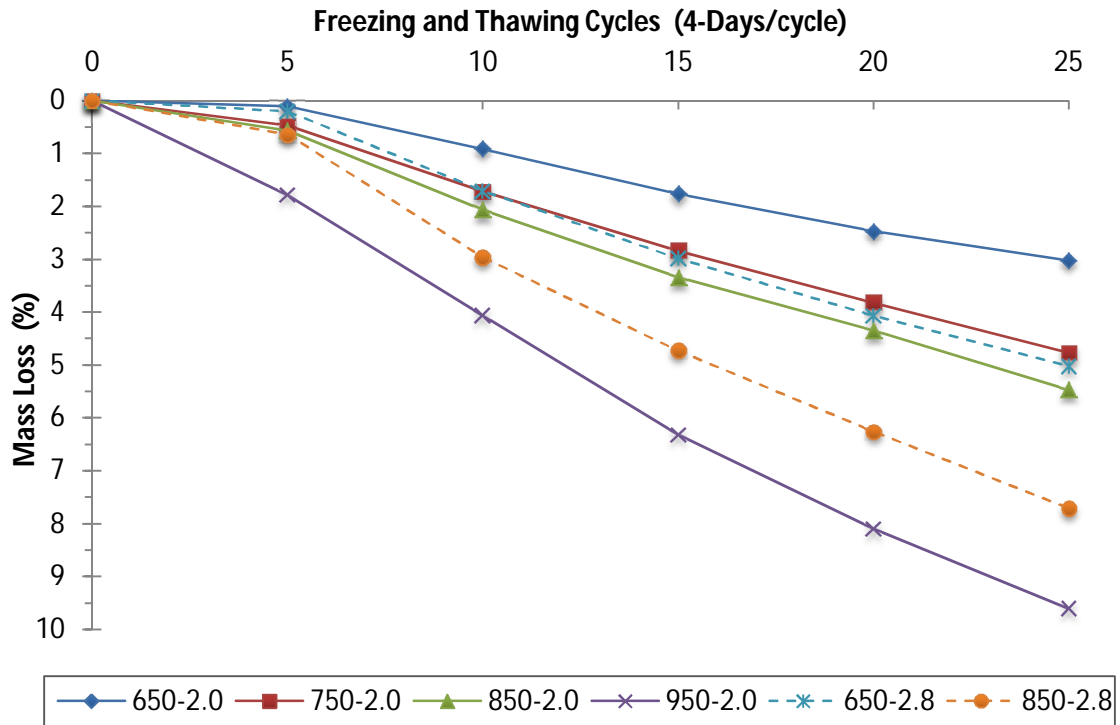
Figure 4-14: Mass Loss of Type V-HES Concretes Tested at the Age of 24 Hrs
