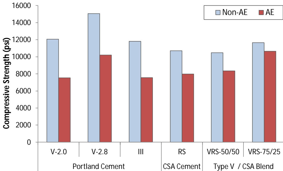
Figure 7-2: Compressive Strength of the Selected HES Concretes at 28 Days
