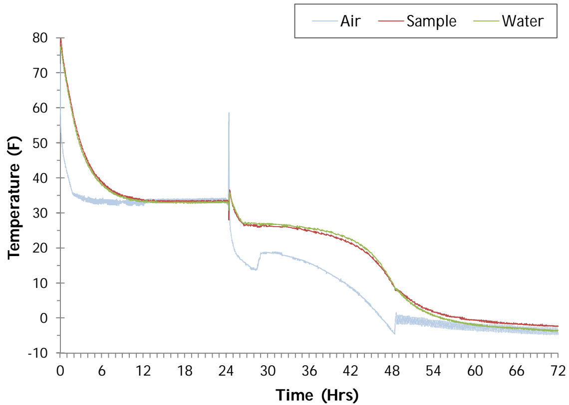
Figure 2-16: Typical Trend for the Cooling of the Freeze/Thaw Samples
