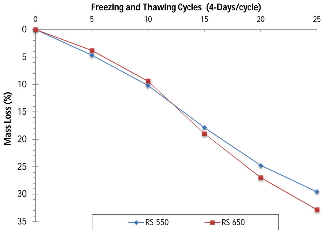
Figure 6-13: Mass Loss of Rapid Set HES Concretes Tested at the Age of 24 Hrs
