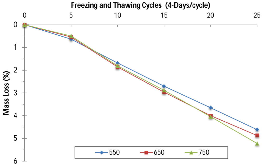
Figure 5-13: Mass Loss of Type III-HES Concretes tested at the Age of 24 Hrs
