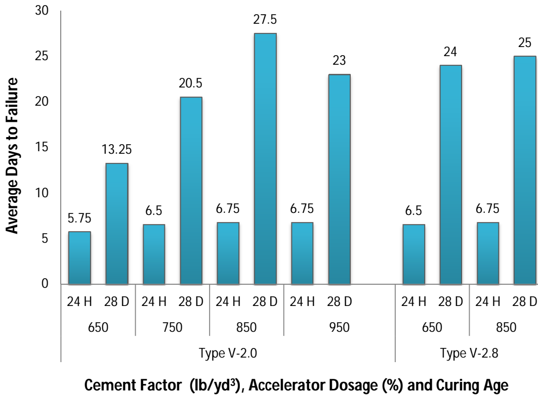
Figure 4-13: Time to Failure for Type V-HES Concretes in Corrosion Test
