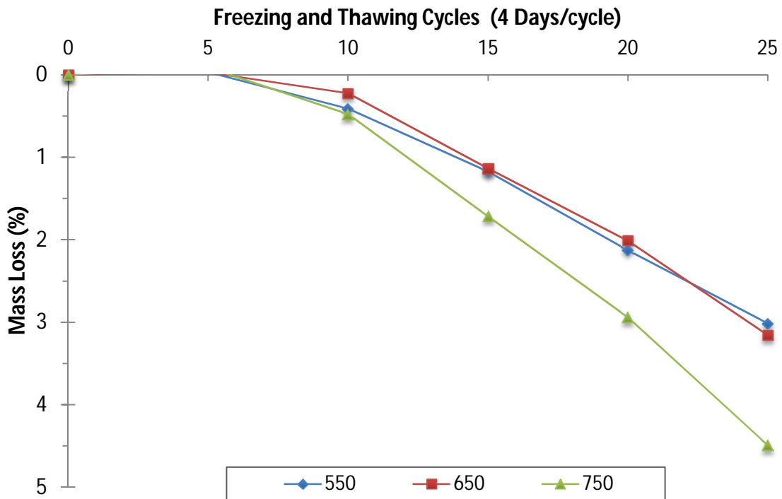
Figure 5-14: Mass Loss of Type III-HES Concretes tested at the Age of 28 Days
