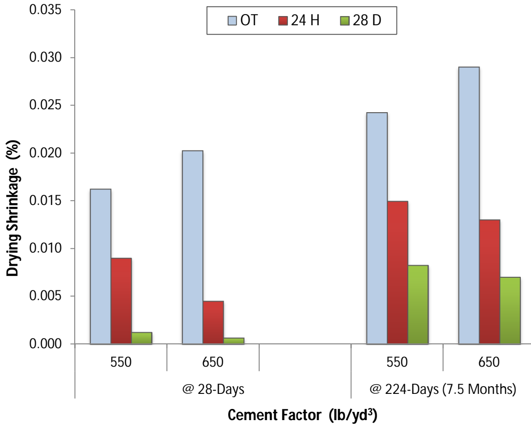
Figure 6-11: The Drying Shrinkage of Rapid Set HES Concretes After 28 Days and 7.5 Months in Shrinkage Room
