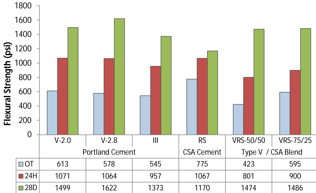
Figure 7-3: Flexural Strength of the Selected HES Concretes
