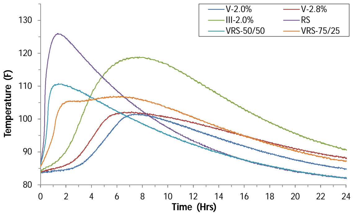
Figure 3-5: Typical Heat of Hydration Trend for Air-Entrained HES Concretes (650 lb/yd 3 )
