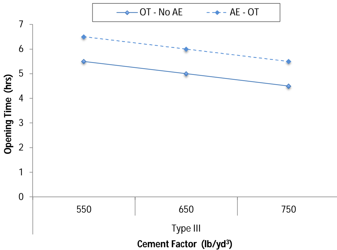
Figure 5-1: Opening Time of Type III-HES Concrete
