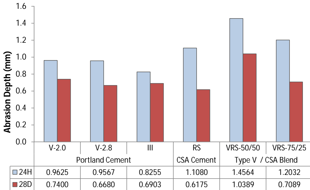
Figure 7-12: Abrasion Depth of the Selected HES Concretes
