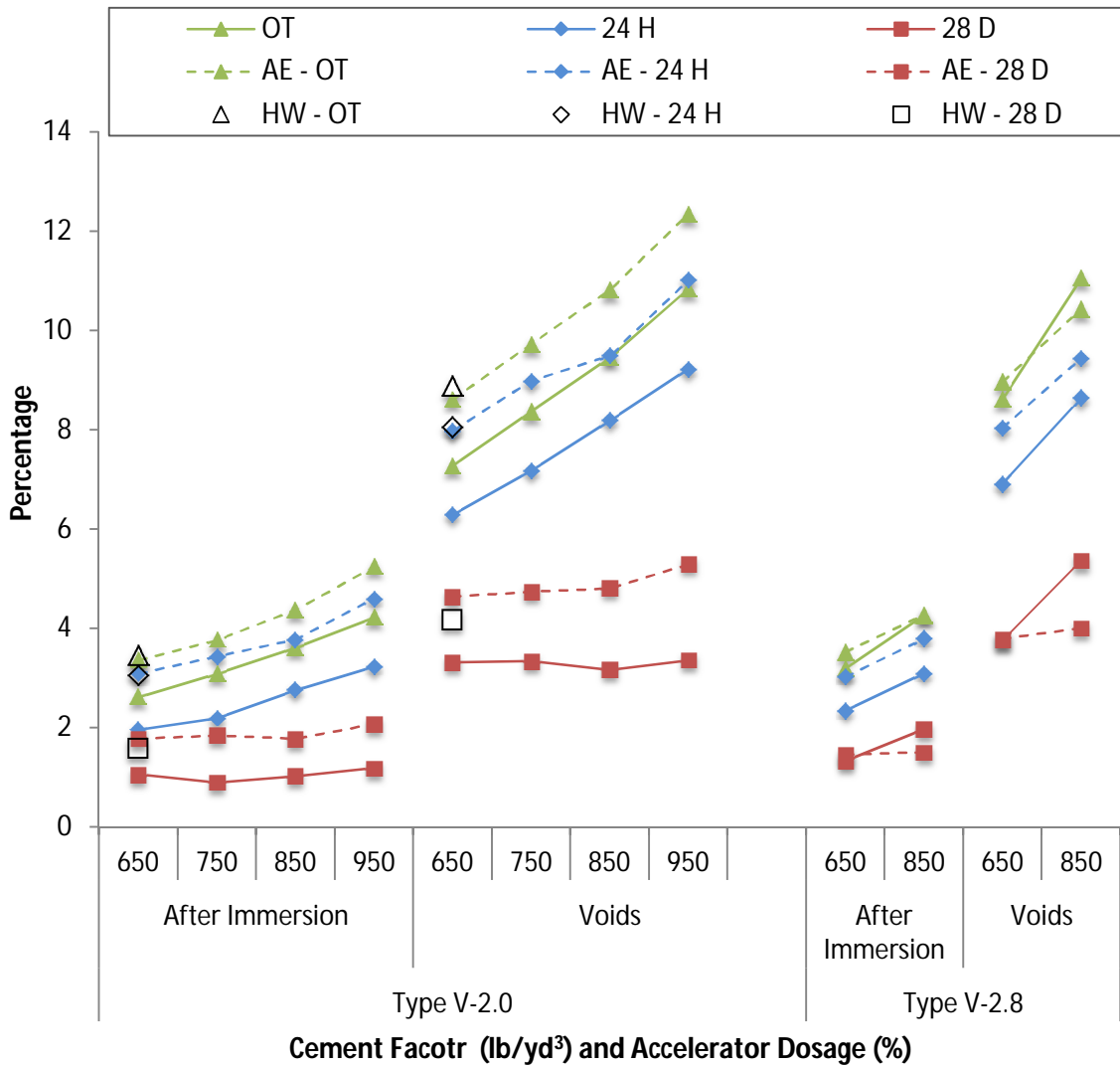
Figure 4-4: Absorption and Volume of Permeable Void for Type V-HES Concretes
