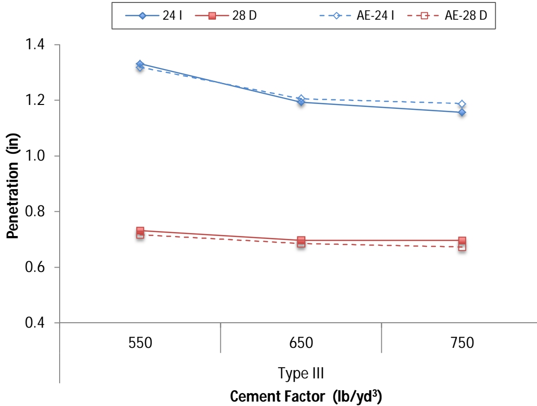
Figure 5-6: Chloride Penetration Depth of Type III-HES Concretes
