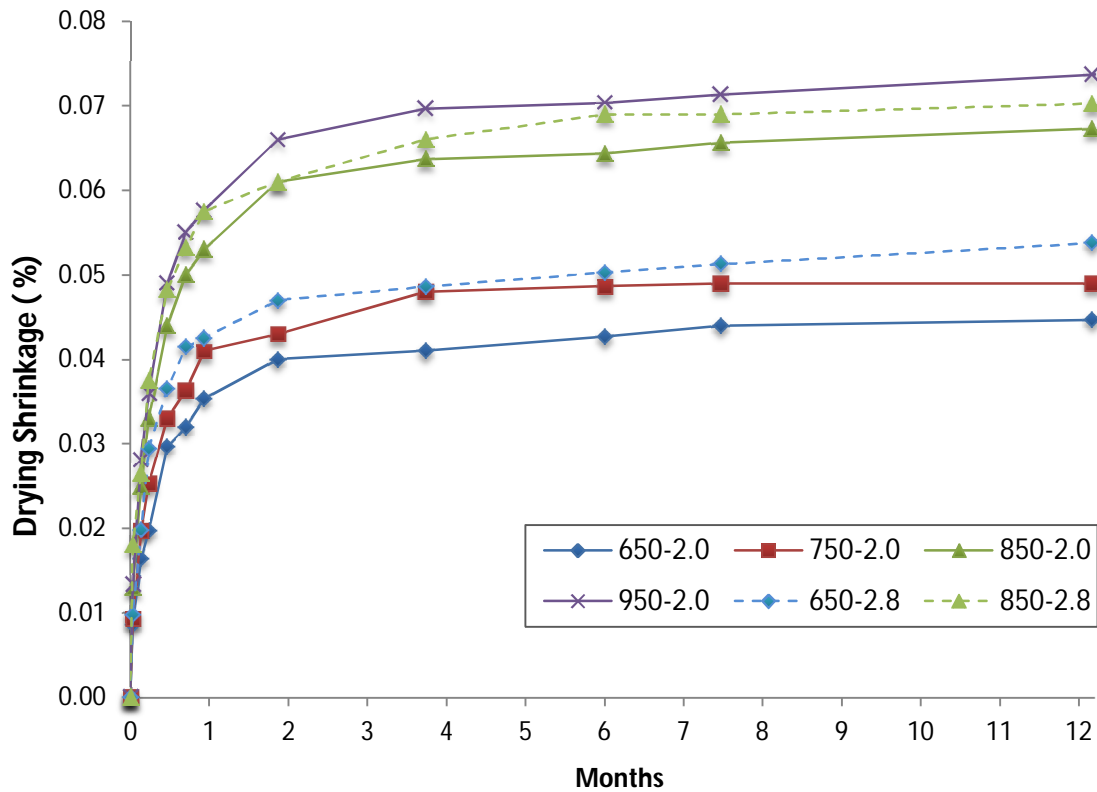
Figure 4-8: Drying Shrinkage of Type V-HES Concretes Transferred to Shrinkage Room at Opening Time
